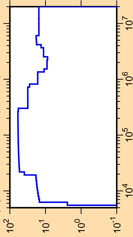
\Delta\mu/\mu vs. E for ^{112}\text{Ru}(\text{mt251})
