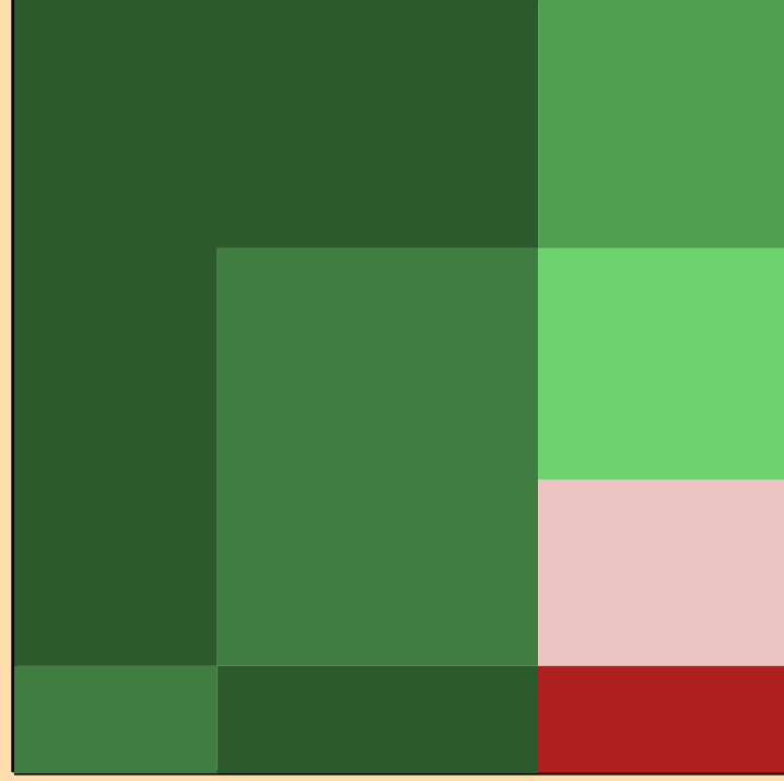
\Delta\sigma/\sigma vs. E for ^{112}\text{Ru}(n,p)
