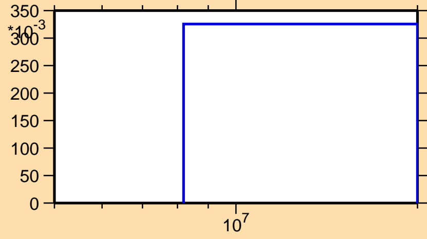
\sigma vs. E for ^{112}\text{Ru}(n,3n)
