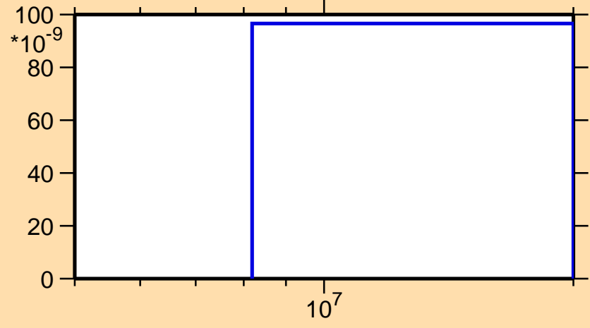
\sigma vs. E for ^{112}\text{Ru}(n,np)
