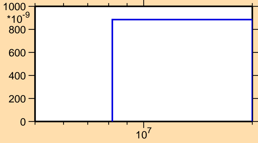
\sigma vs. E for ^{112}\text{Ru}(n,\alpha)
