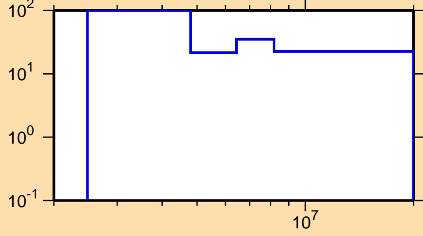
\Delta\sigma/\sigma vs. E for ^{112}\text{Ru}(n,n\text{cont.})
