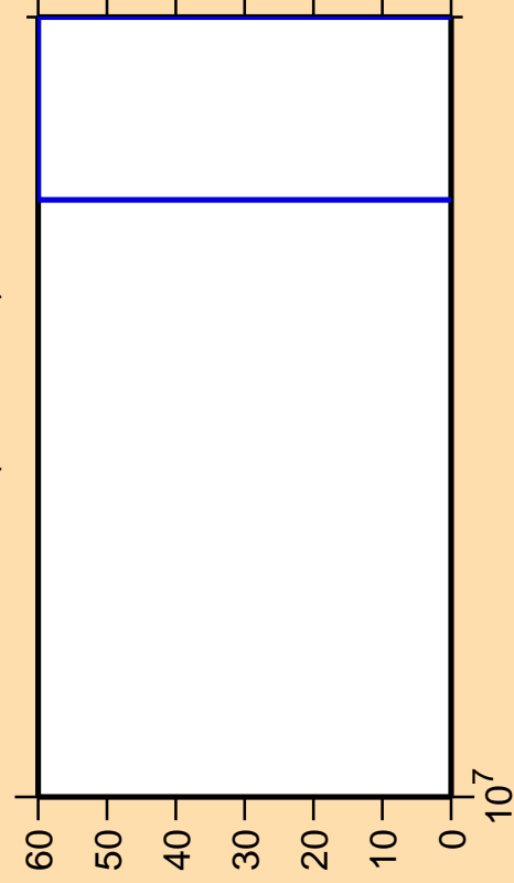
\Delta\sigma/\sigma vs. E for ^{30}\text{S}(n,ncont.)
