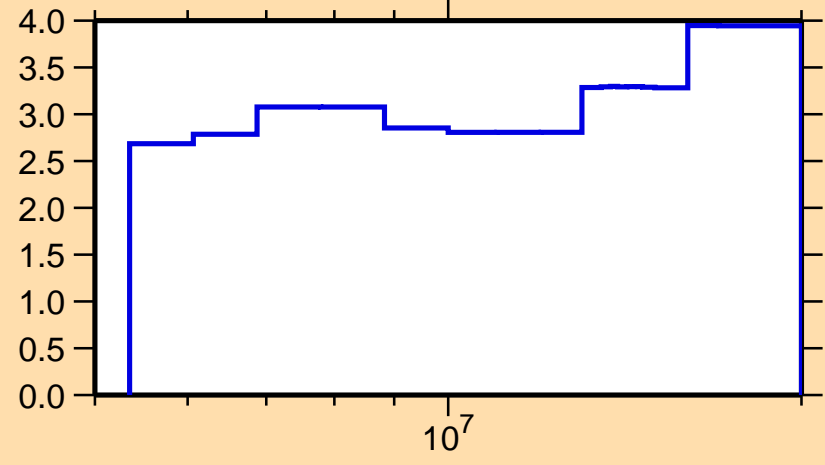
\Delta\sigma/\sigma vs. E for ^{30}\text{S}(n,n\text{onel.})
