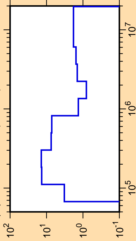
\Delta\mu/\mu vs. E for ^{30}\text{S}(\text{mt251})
