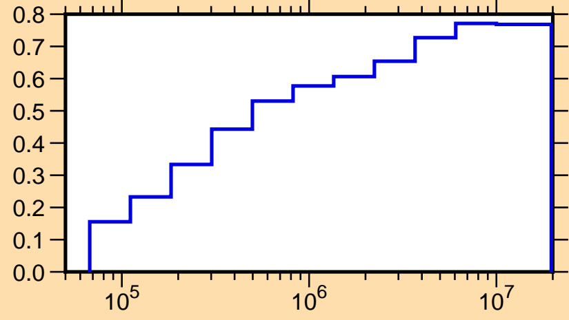
\mu vs. E for ^{30}\text{S}(\text{mt251})
