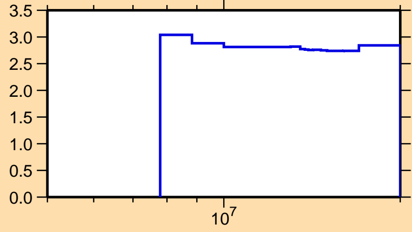
\Delta\sigma/\sigma vs. E for ^{32}\text{S}(n,n\text{onel.})
