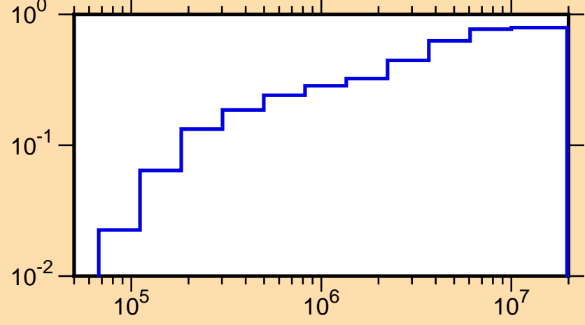
\mu vs. E for ^{32}\text{S}(\text{mt251})
