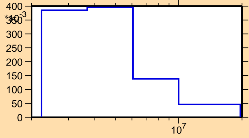
\sigma vs. E for ^{32}\text{S}(n,n_1)
