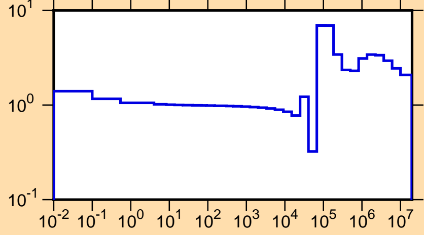
\sigma vs. E for ^{32}\text{S}(n,\text{tot.})
