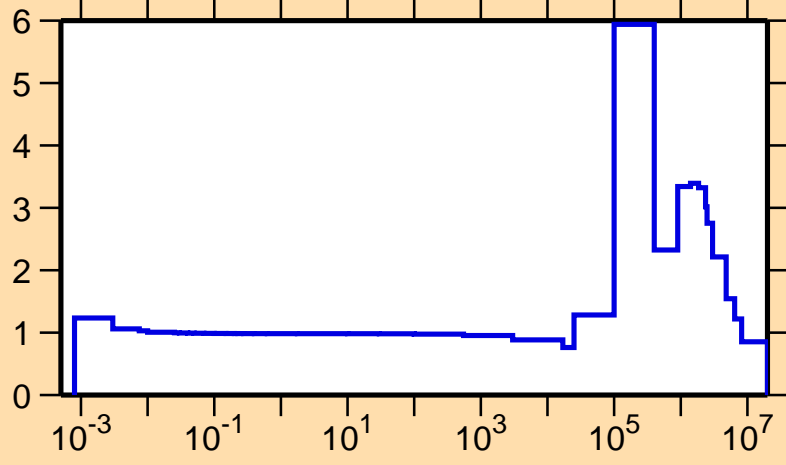
\sigma vs. E for ^{32}\text{S}(n,\text{el.})
