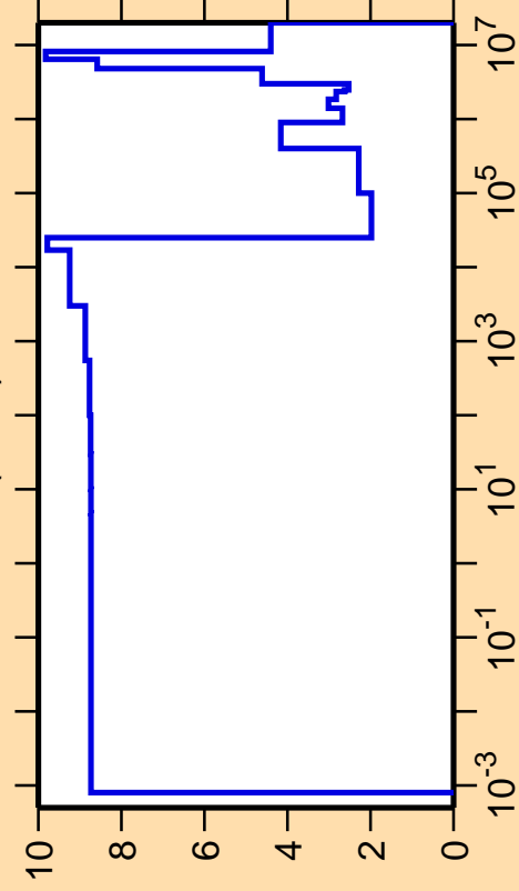
\Delta\sigma/\sigma vs. E for ^{32}\text{S}(n,\text{el.})
