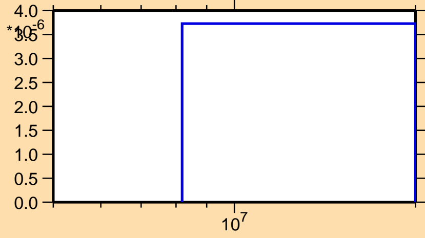
\sigma vs. E for ^{32}\text{S}(n,\text{pd})
