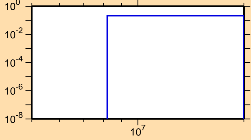
\sigma vs. E for ^{32}\text{S}(n,n\alpha)
