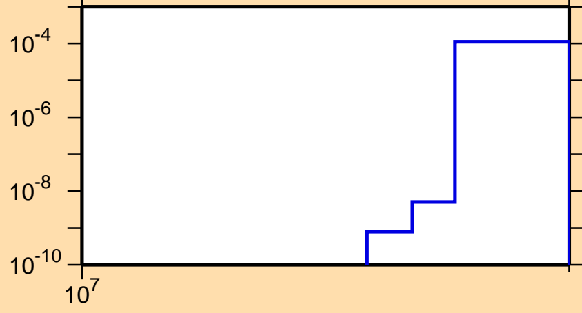
\sigma vs. E for ^{35}\text{S}(n,2n\alpha)
