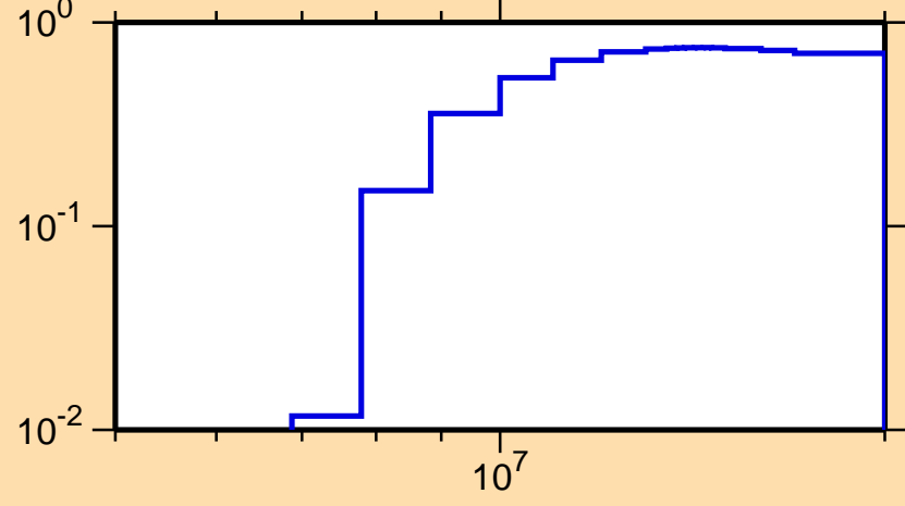
\sigma vs. E for ^{35}\text{S}(n,2n)
