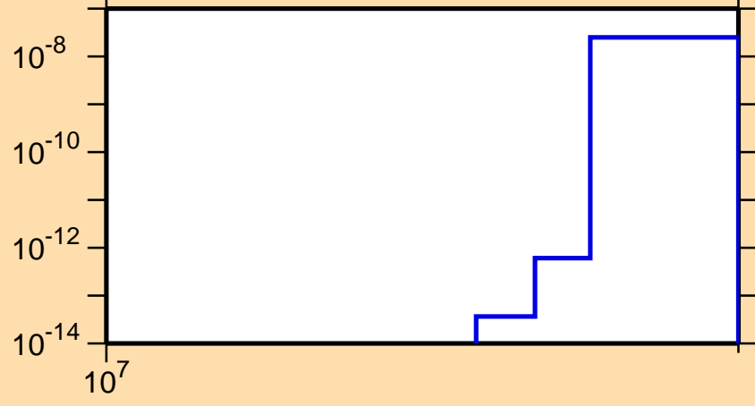
\sigma vs. E for ^{35}\text{S}(n,\text{He}3)
