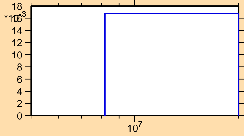
\sigma vs. E for ^{35}\text{S}(n,n\alpha)
