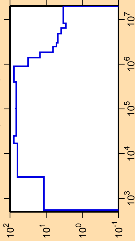
\Delta\sigma/\sigma vs. E for ^{35}\text{S}(n,\text{nonel.})
