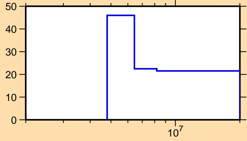
\Delta\sigma/\sigma vs. E for ^{35}\text{S}(n,ncont.)
