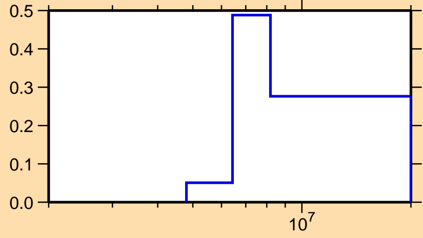
\sigma vs. E for ^{35}\text{S}(n,n\text{cont.})
