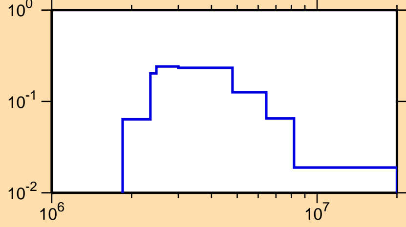
\sigma vs. E for ^{35}\text{S}(n,n_2)
