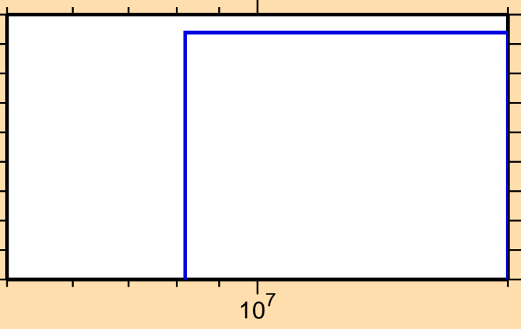
\sigma vs. E for ^{35}\text{S}(n,n\alpha)
