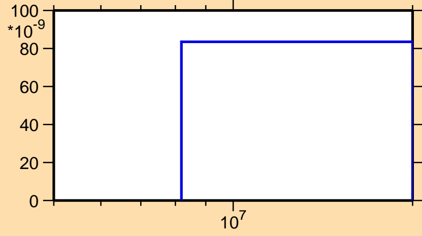
\sigma vs. E for ^{35}\text{S}(n,3n)
