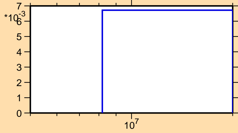
\sigma vs. E for ^{35}\text{S}(n,np)
