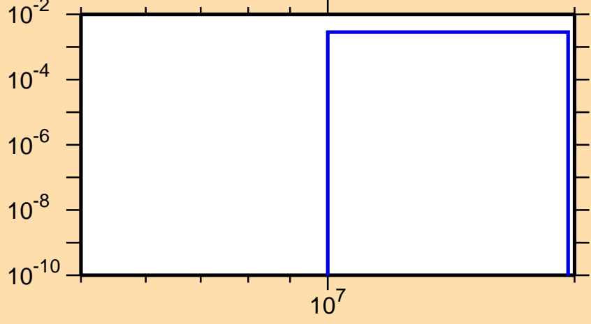
\sigma vs. E for ^{36}\text{S}(n,n\alpha)
