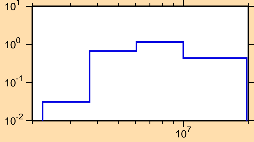
\sigma vs. E for ^{36}\text{S}(n,\text{inel.})
