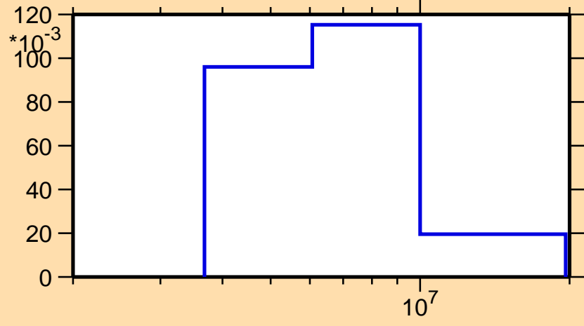
\sigma vs. E for ^{36}\text{S}(n,n_3)
