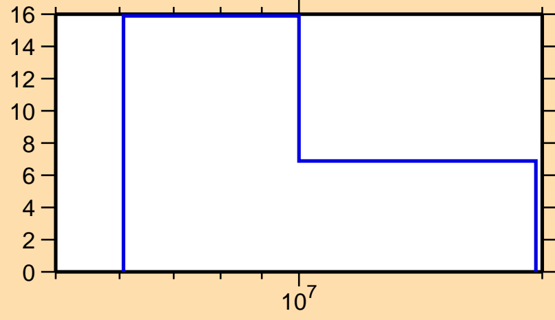
\Delta\sigma/\sigma vs. E for ^{36}\text{S}(n,el.)
