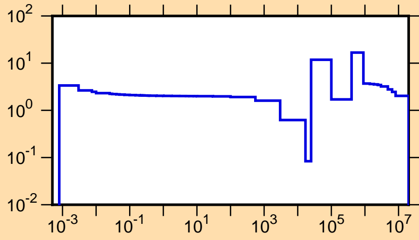
\sigma vs. E for ^{36}\text{S}(n,\text{tot.})
