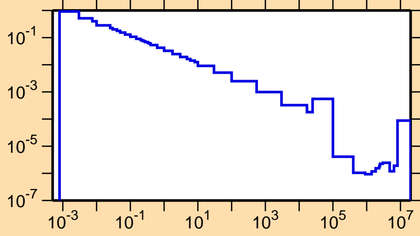
\sigma vs. E for ^{36}\text{S}(n,\gamma)
