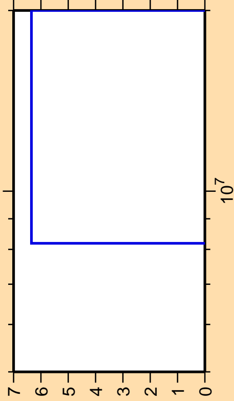
\Delta\sigma/\sigma vs. E for ^{36}\text{S}(n,nd)
