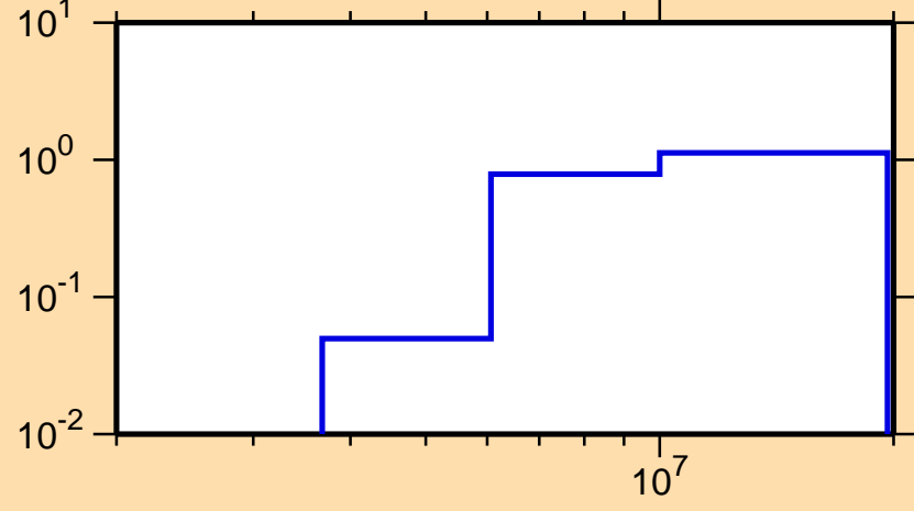
\sigma vs. E for ^{37}\text{S}(n,2n)
