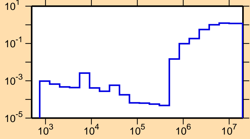
\sigma vs. E for ^{37}\text{S}(n,\text{nonel.})
