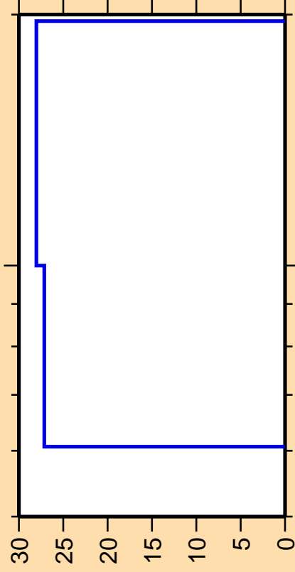
\Delta\sigma/\sigma vs. E for ^{37}\text{S}(n,p)
