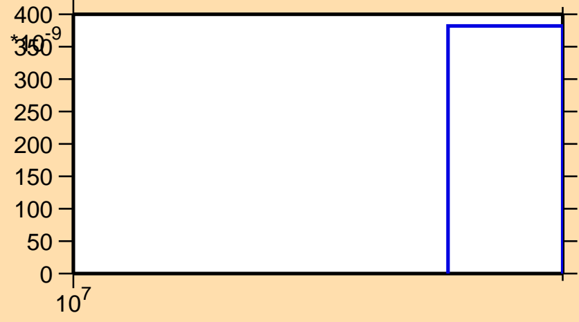
\sigma vs. E for ^{38}\text{S}(n,nt)
