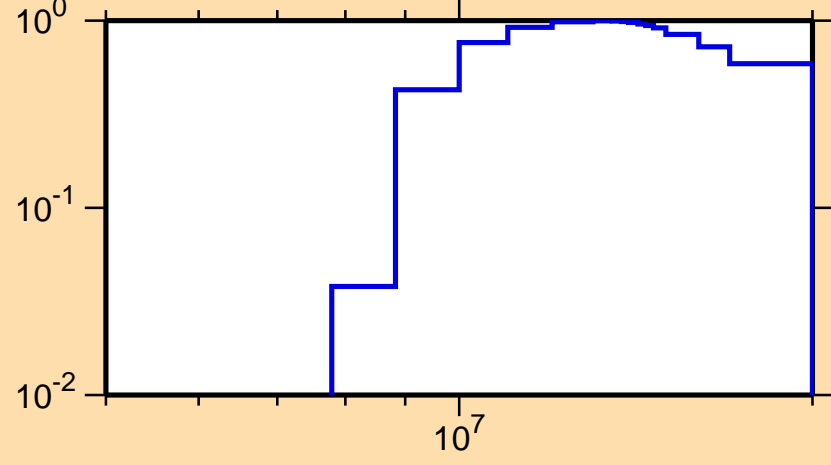
\sigma vs. E for ^{38}\text{S}(n,2n)
