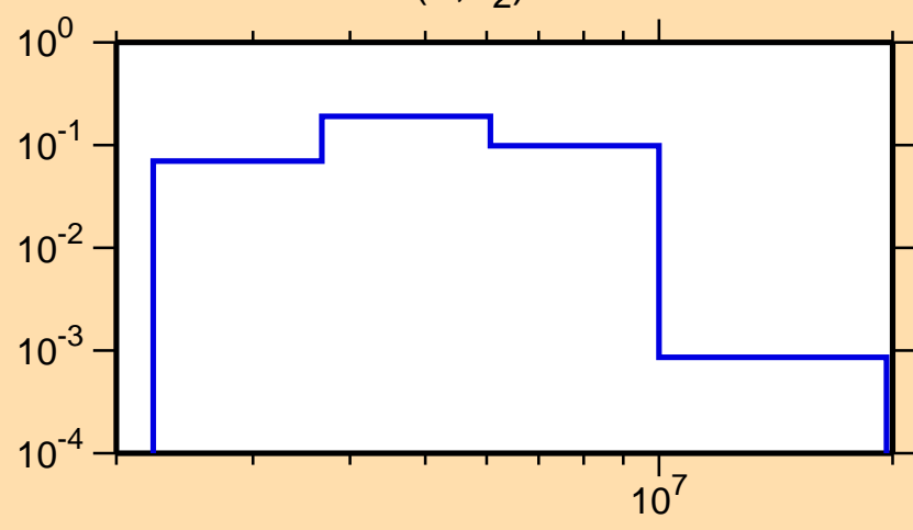
\sigma vs. E for ^{38}\text{S}(n,n_2)
