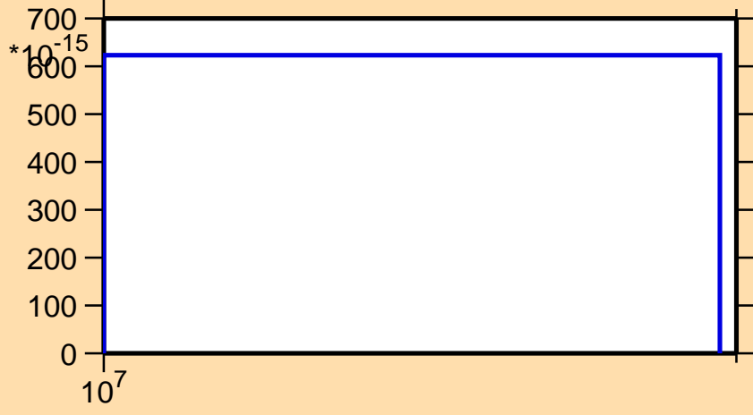
\sigma vs. E for ^{38}\text{S}(n,2n\alpha)
