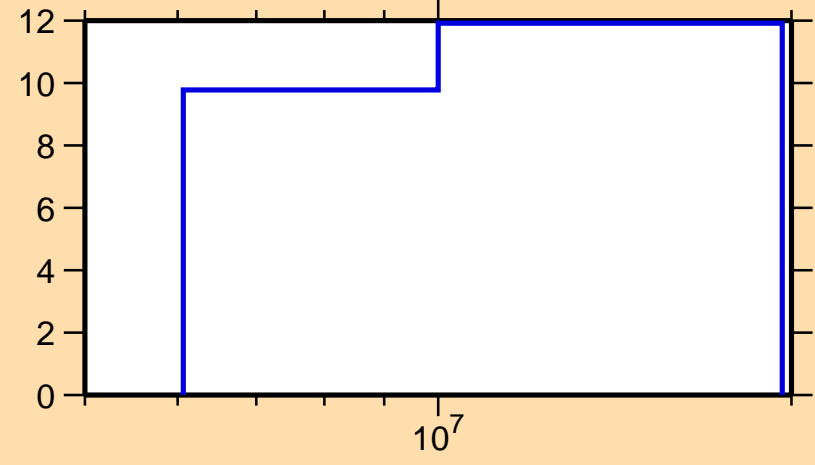
\Delta\sigma/\sigma vs. E for ^{38}\text{S}(n,n\text{onel.})
