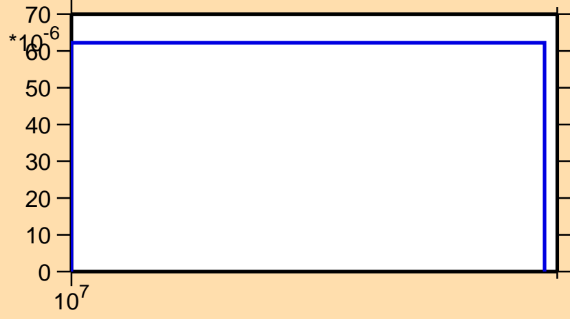
\sigma vs. E for ^{38}\text{S}(n,d)
