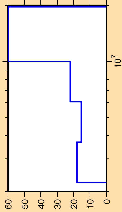
\Delta\sigma/\sigma vs. E for ^{38}\text{S}(n,n_3)
