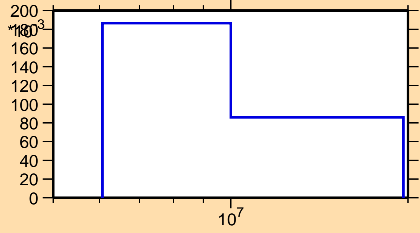
\sigma vs. E for ^{38}\text{S}(n,n\text{cont.})
