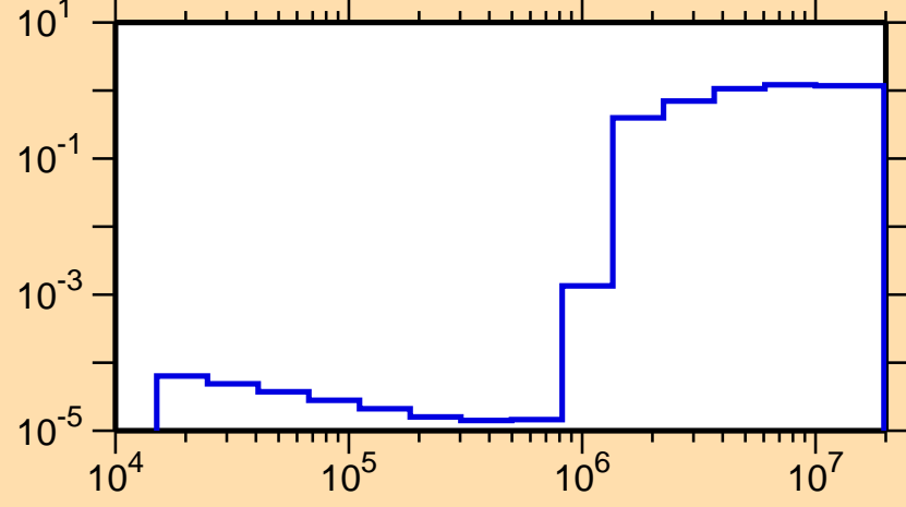
\sigma vs. E for ^{38}\text{S}(n,\text{nonel.})
