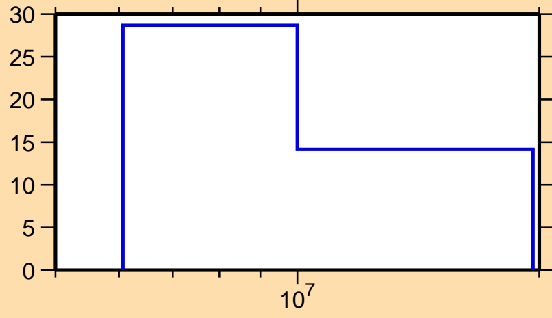
\Delta\sigma/\sigma vs. E for ^{38}\text{S}(n,\text{el.})
