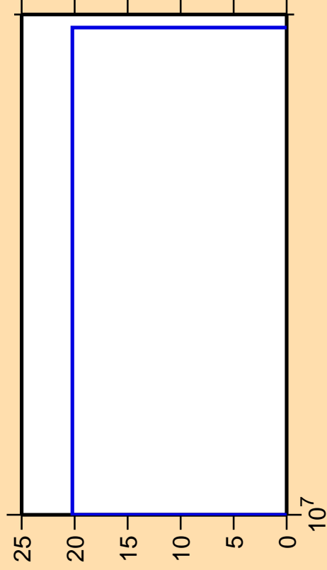
\Delta\sigma/\sigma vs. E for ^{38}\text{S}(n,3n)
