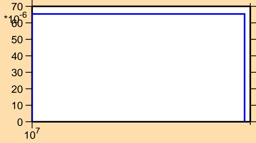
\sigma vs. E for ^{38}\text{S}(n,p)
