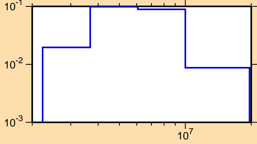
\sigma vs. E for ^{38}\text{S}(n,n_3)
