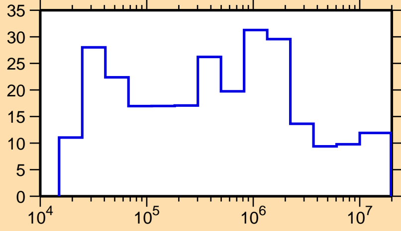
\Delta\sigma/\sigma vs. E for ^{38}\text{S}(n,\text{nonel.})
