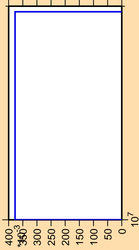
\Delta\sigma/\sigma vs. E for ^{38}\text{S}(n,2n\alpha)
