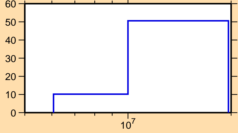
\Delta\sigma/\sigma vs. E for ^{38}\text{S}(n,\text{inel.})
