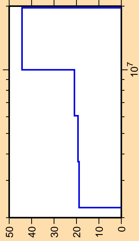
\Delta\sigma/\sigma vs. E for ^{38}\text{S}(n,n_2)
