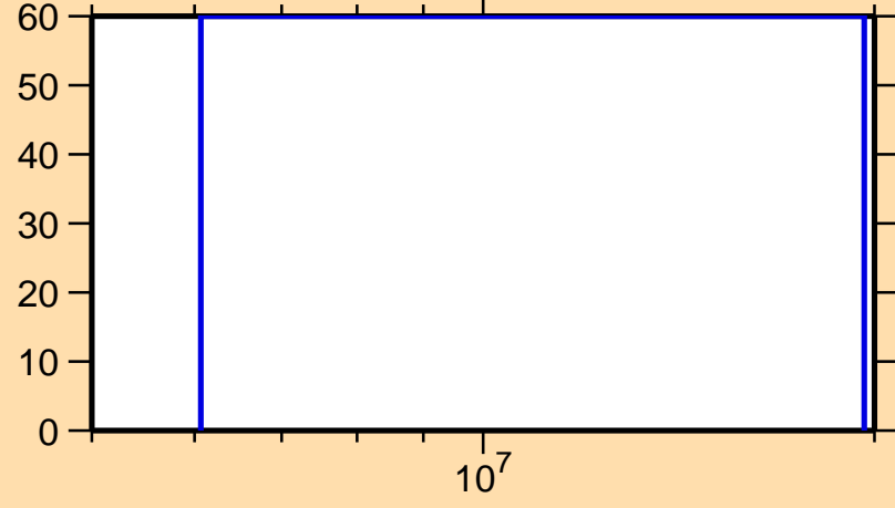
\Delta\sigma/\sigma vs. E for ^{38}\text{S}(n,\gamma)
