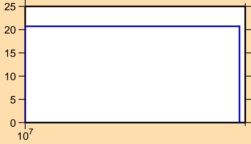
\Delta\sigma/\sigma vs. E for ^{38}\text{S}(n,2n)
