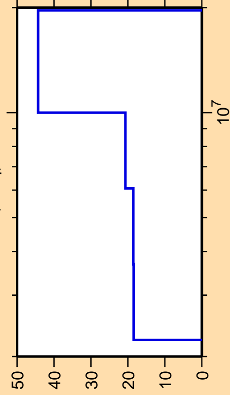
\Delta\sigma/\sigma vs. E for ^{38}\text{S}(n,n_4)
