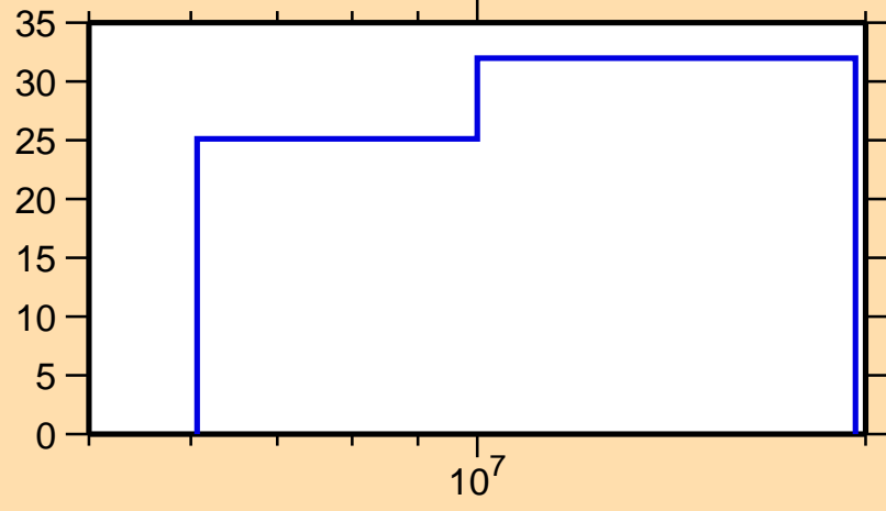
\Delta\sigma/\sigma vs. E for ^{38}\text{S}(n,n\text{cont.})
