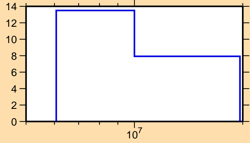
\Delta\sigma/\sigma vs. E for ^{38}\text{S}(n,\text{tot.})
