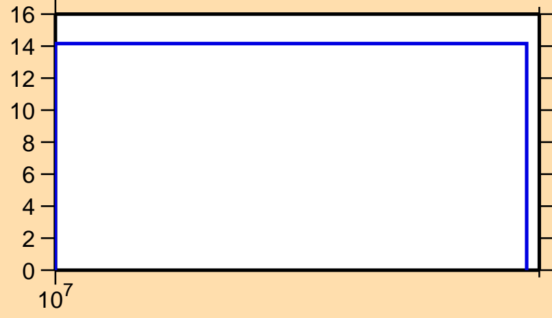
\Delta\sigma/\sigma vs. E for ^{38}\text{S}(n,el.)
