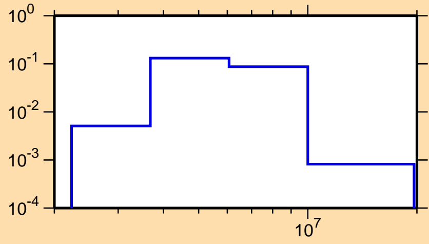
\sigma vs. E for ^{38}\text{S}(n,n_4)
