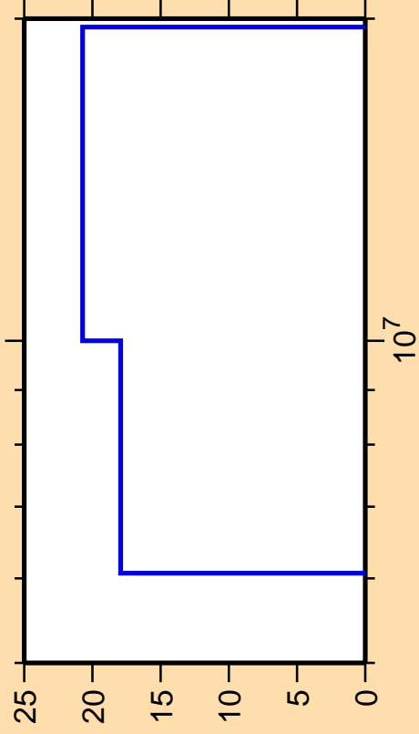
\Delta\sigma/\sigma vs. E for ^{38}\text{S}(n,2n)
