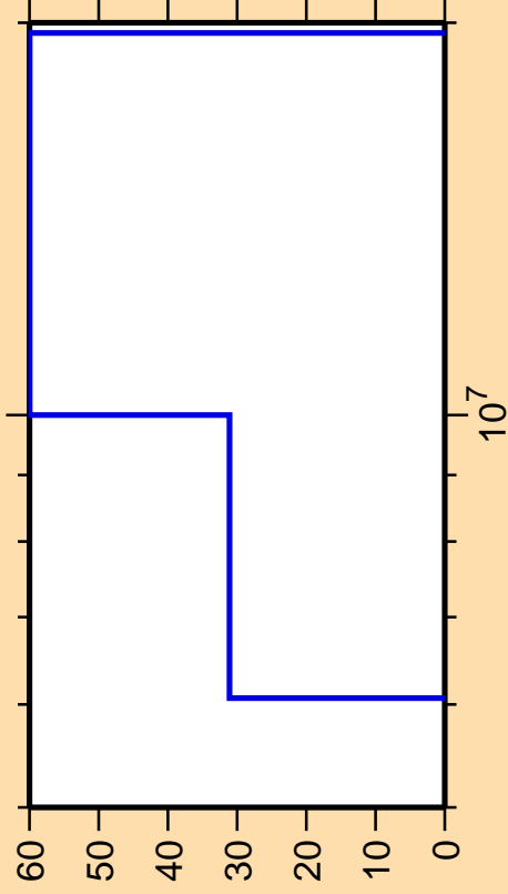
\Delta\sigma/\sigma vs. E for ^{38}\text{S}(n,\alpha)
