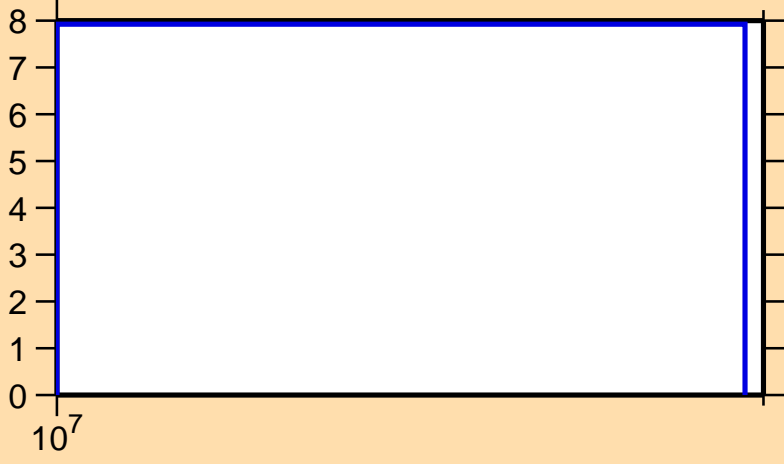
\Delta\sigma/\sigma vs. E for ^{38}\text{S}(n,\text{tot.})
