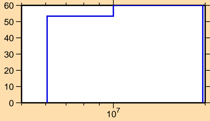
\Delta\sigma/\sigma vs. E for ^{38}\text{S}(n,n_1)
