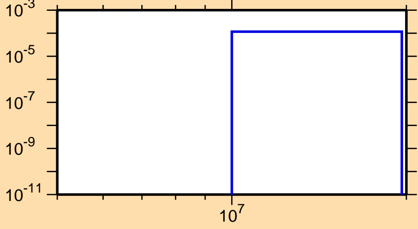
\sigma vs. E for ^{38}\text{S}(n,n\alpha)
