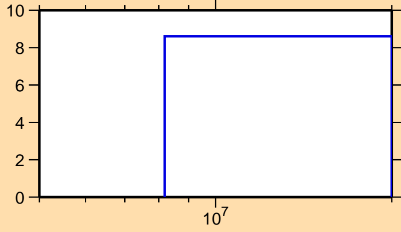
\Delta\sigma/\sigma vs. E for ^{38}\text{S}(n,tot.)
