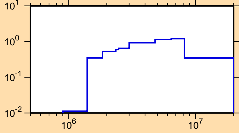
\sigma vs. E for ^{38}\text{S}(n,\text{inel.})
