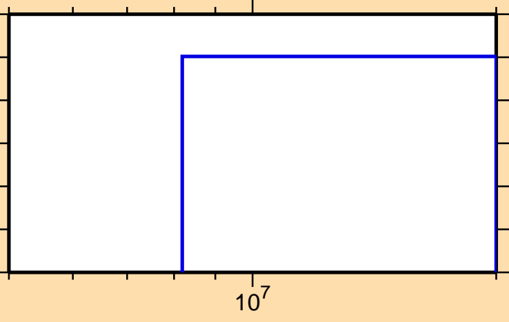
\sigma vs. E for ^{38}\text{S}(n,d)
