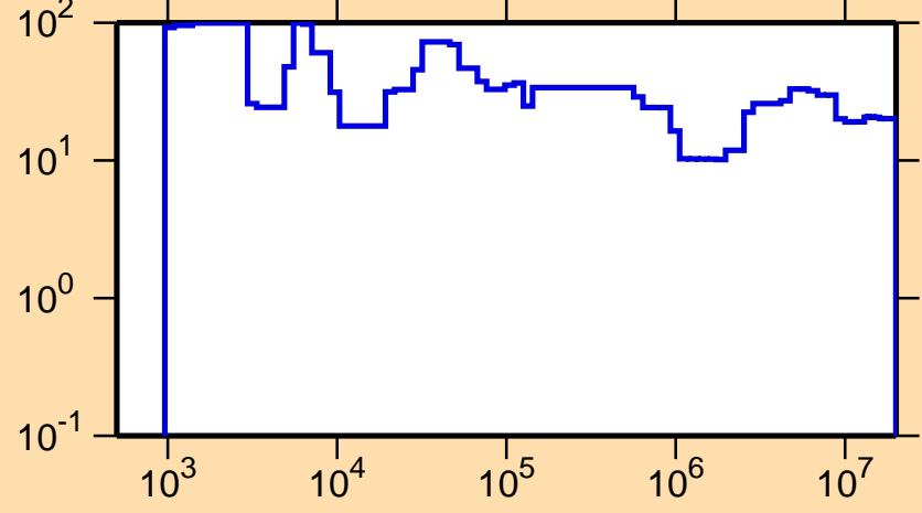
\Delta\sigma/\sigma vs. E for ^{39}\text{S}(n,\text{el.})
