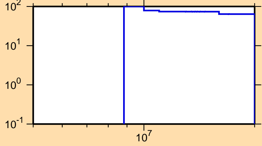
\Delta\sigma/\sigma vs. E for ^{39}\text{S}(n,p)
