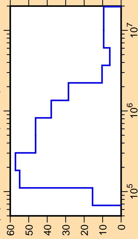
\Delta\mu/\mu vs. E for ^{39}\text{S}(\text{mt251})
