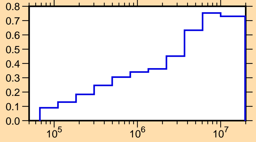
\mu vs. E for ^{39}\text{S}(\text{mt251})
