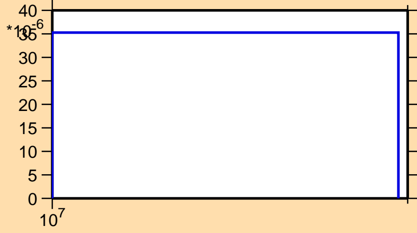
\sigma vs. E for ^{39}\text{S}(n,t)
