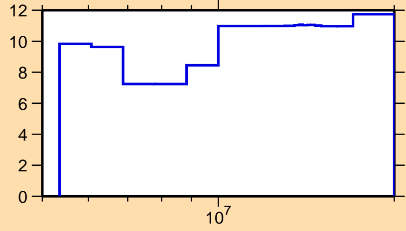
\Delta\sigma/\sigma vs. E for ^{40}\text{S}(n,n\text{onel.})
