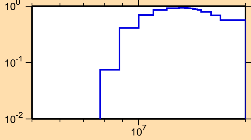
\sigma vs. E for ^{40}\text{S}(n,2n)
