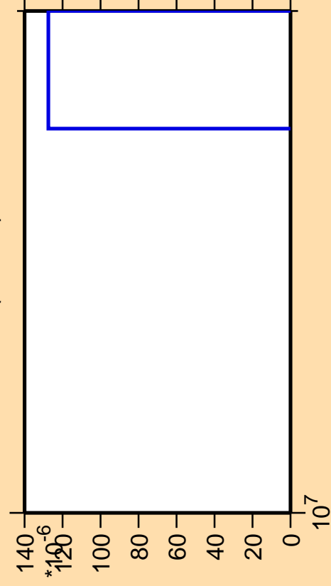
\Delta\sigma/\sigma vs. E for ^{40}\text{S}(n,2n\alpha)
