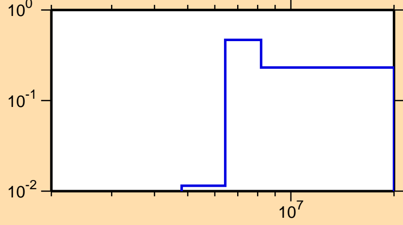
\sigma vs. E for ^{40}\text{S}(n,n\text{cont.})
