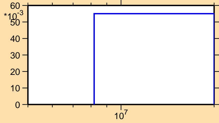
\sigma vs. E for ^{40}\text{S}(n,3n)
