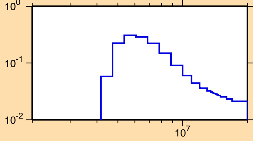
\sigma vs. E for ^{41}\text{S}(n,n\text{cont.})
