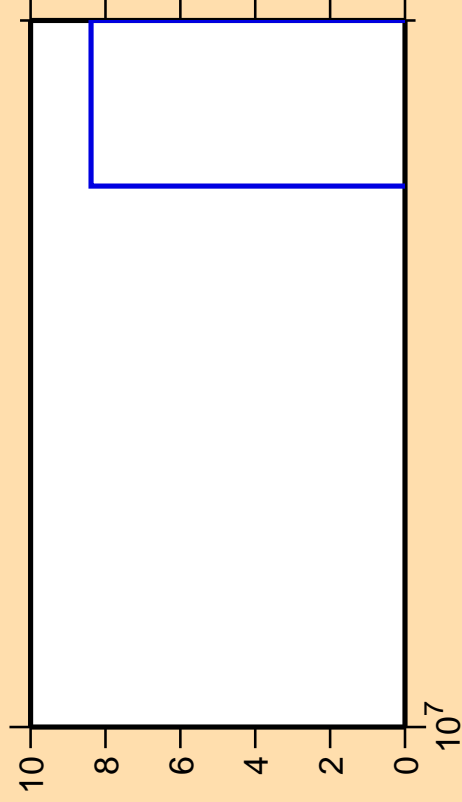
\Delta\sigma/\sigma vs. E for ^{41}\text{S}(n,nt)
