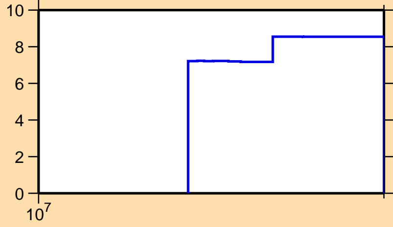
\Delta\sigma/\sigma vs. E for ^{41}\text{S}(n,el.)
