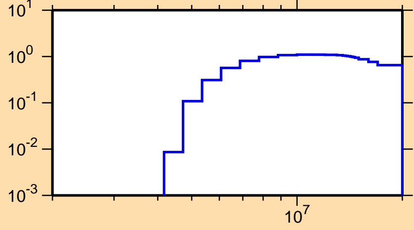
\sigma vs. E for ^{41}\text{S}(n,2n)
