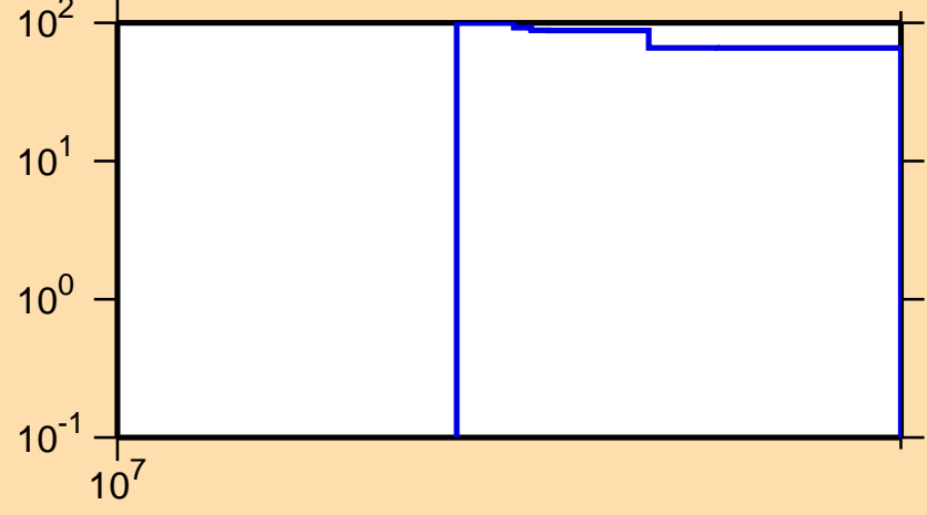
\Delta\sigma/\sigma vs. E for ^{41}\text{S}(n,p)
