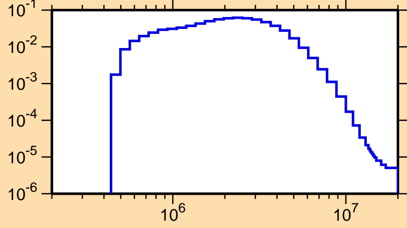
\sigma vs. E for ^{41}\text{S}(n,n_1)
