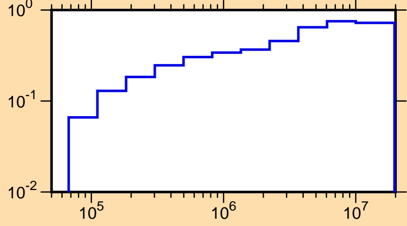
\mu vs. E for ^{41}\text{S}(\text{mt251})
