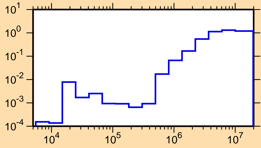
\sigma vs. E for ^{41}\text{S}(n,\text{nonel.})
