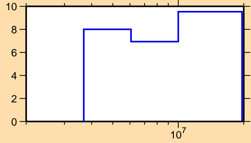
\Delta\sigma/\sigma vs. E for ^{41}\text{S}(n,n\text{onel.})
