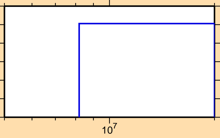
\sigma vs. E for ^{41}\text{S}(n,\alpha)
