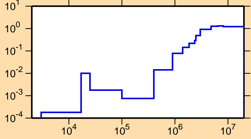
\sigma vs. E for ^{41}\text{S}(n,\text{nonel.})
