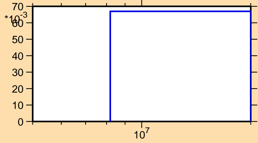
\sigma vs. E for ^{41}\text{S}(n,3n)
