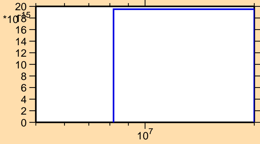
\sigma vs. E for ^{41}\text{S}(n,nt)
