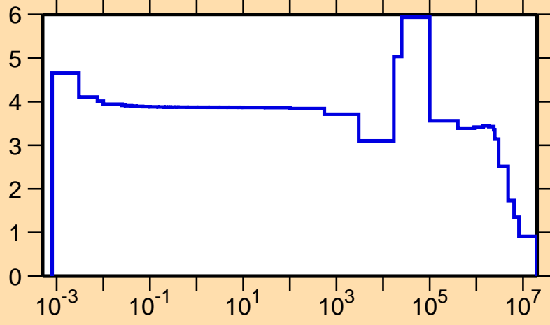
\sigma vs. E for ^{41}\text{S}(n,\text{el.})
