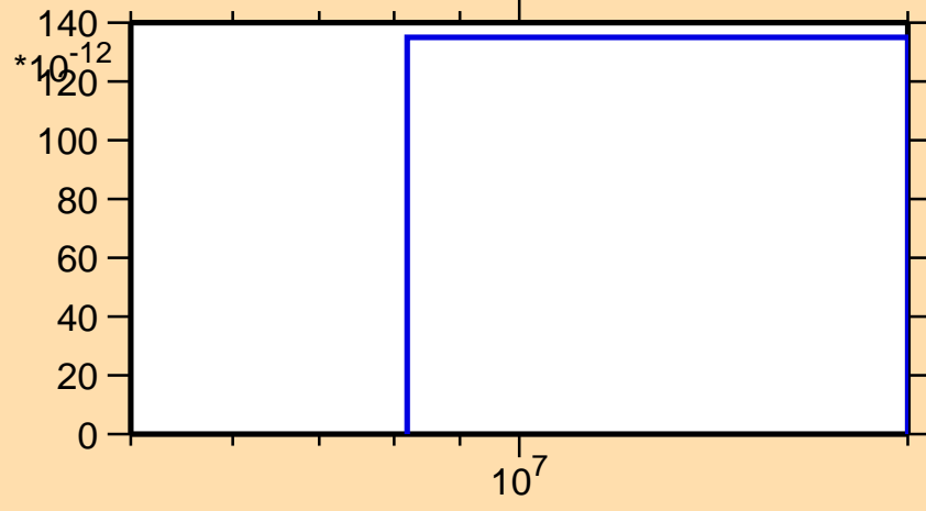
\sigma vs. E for ^{41}\text{S}(n,np)
