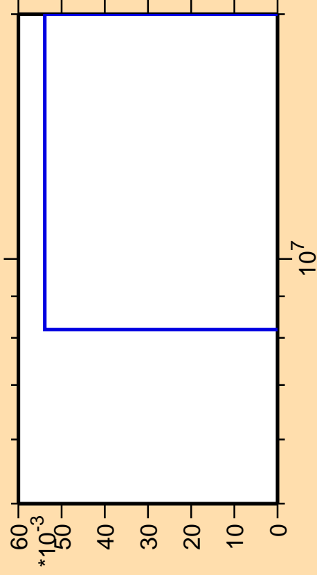
\Delta\sigma/\sigma vs. E for ^{41}\text{S}(n,\text{nd})
