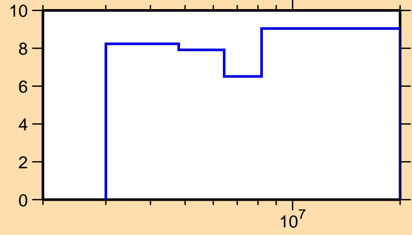
\Delta\sigma/\sigma vs. E for ^{41}\text{S}(n,n\text{nonel.})
