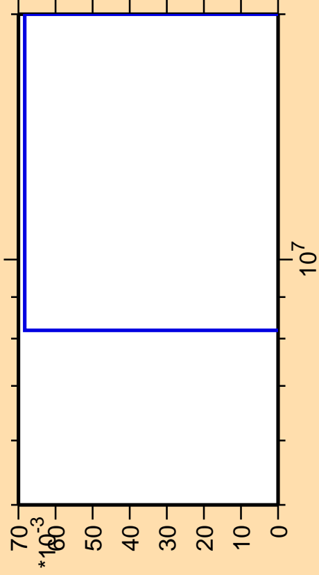
\Delta\sigma/\sigma vs. E for ^{41}\text{S}(n,nt)
