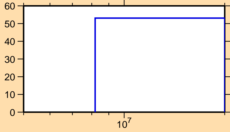
\Delta\sigma/\sigma vs. E for ^{41}\text{S}(n,ncont.)
