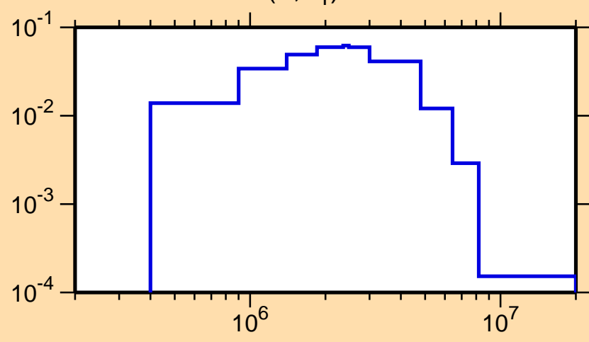
\sigma vs. E for ^{41}\text{S}(n,n_1)
