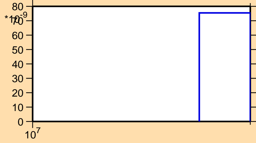
\sigma vs. E for ^{42}\text{S}(n,d)
