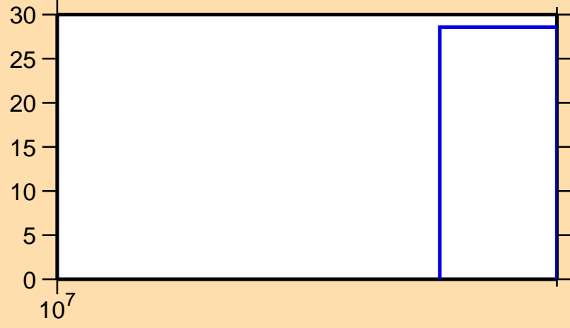
\Delta\sigma/\sigma vs. E for ^{42}\text{S}(n,el.)
