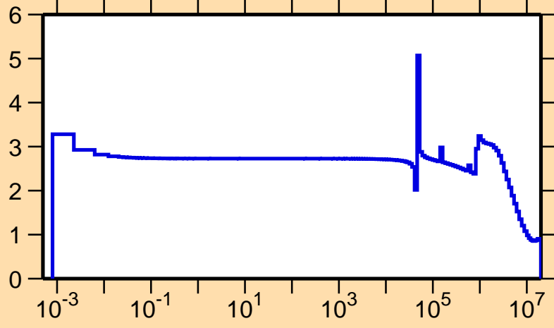
\sigma vs. E for ^{42}\text{S}(n,\text{el.})
