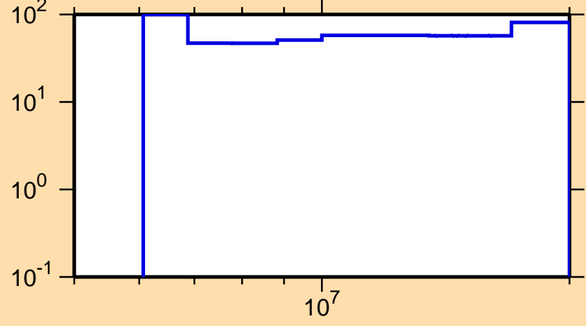
\Delta\sigma/\sigma vs. E for ^{42}\text{S}(n,2n)
