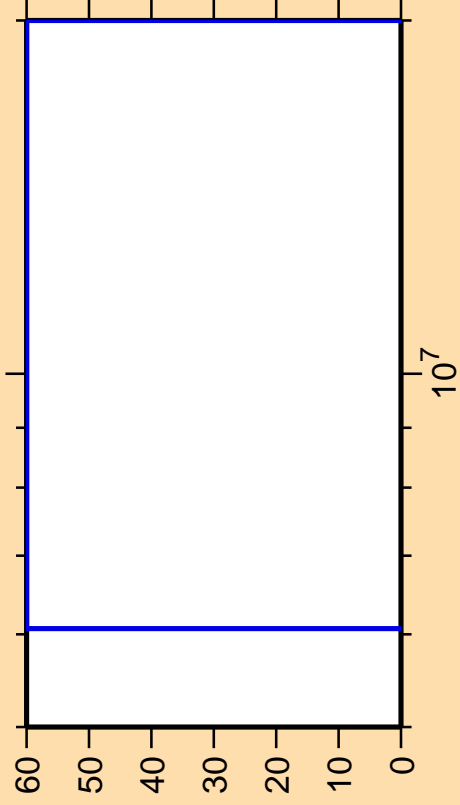
\Delta\sigma/\sigma vs. E for ^{42}\text{S}(n,n_1)
