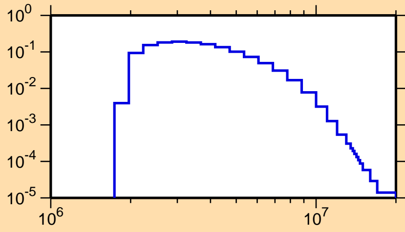
\sigma vs. E for ^{42}\text{S}(n,n_2)
