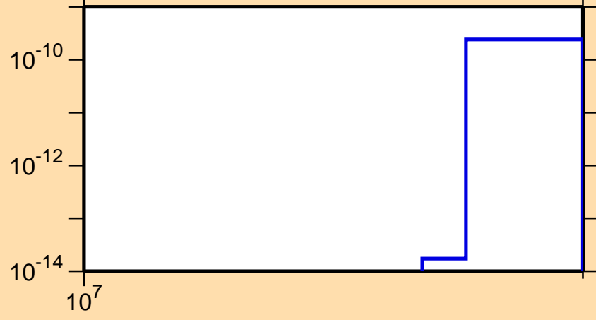
\sigma vs. E for ^{42}\text{S}(n,n\alpha)
