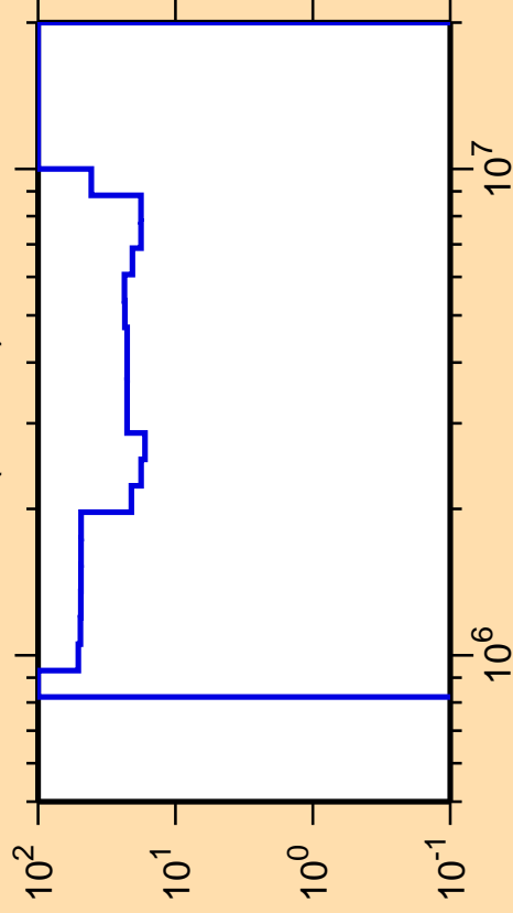
\Delta\sigma/\sigma vs. E for ^{42}\text{S}(n,\text{inel.})
