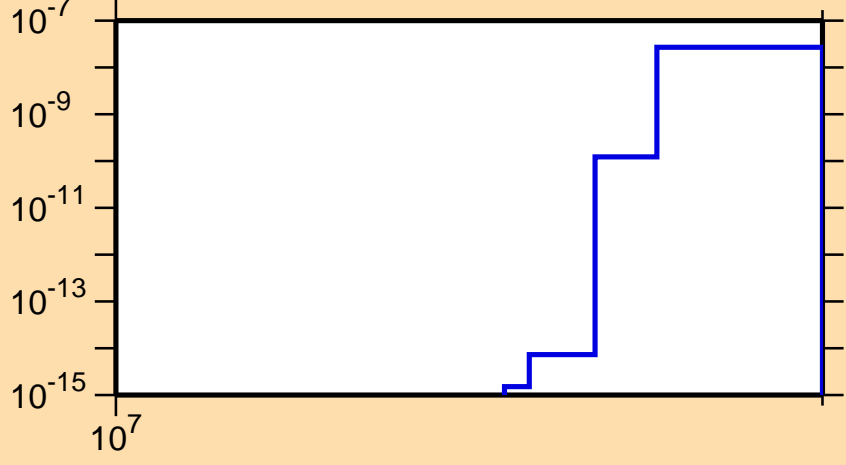
\sigma vs. E for ^{42}\text{S}(n,\alpha)
