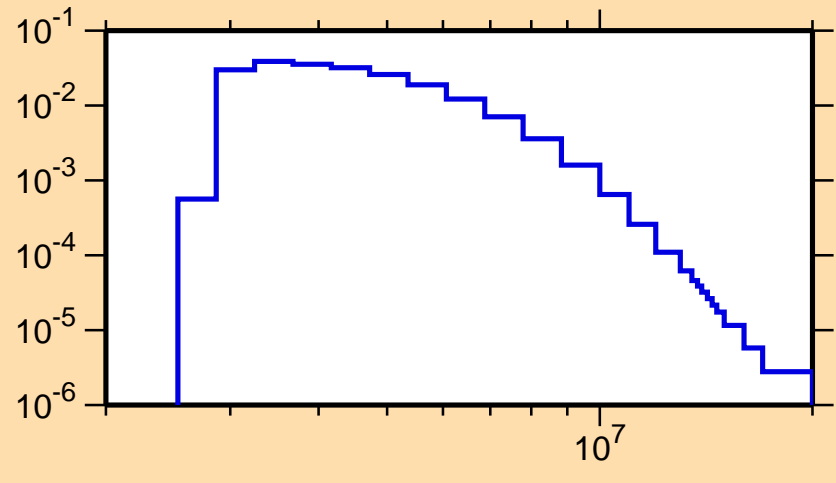
\sigma vs. E for ^{42}\text{S}(n,n_4)
