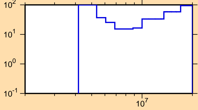
\Delta\sigma/\sigma vs. E for ^{42}\text{S}(n,n\text{cont.})
