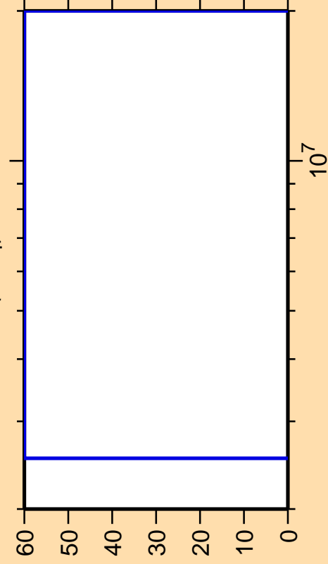
\Delta\sigma/\sigma vs. E for ^{42}\text{S}(n,n_4)
