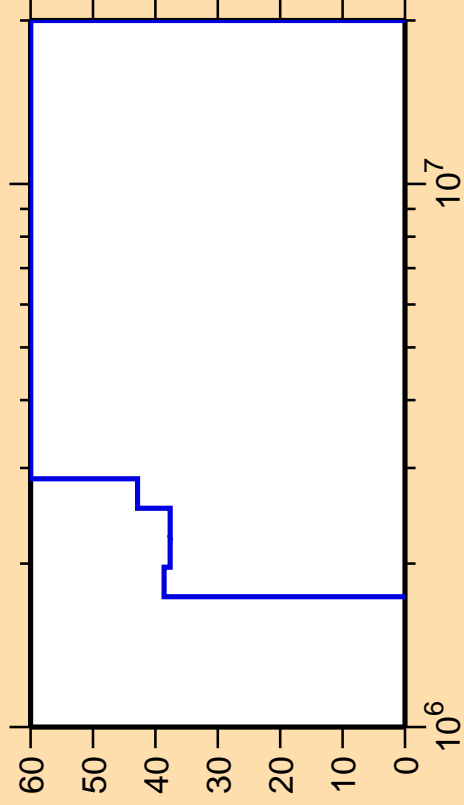
\Delta\sigma/\sigma vs. E for ^{42}\text{S}(n,n_2)
