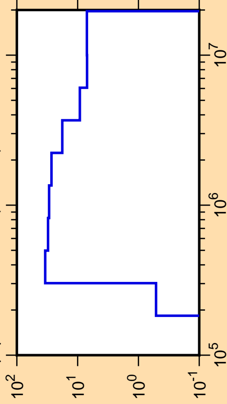
\Delta\mu/\mu vs. E for ^{42}\text{S}(\text{mt251})
