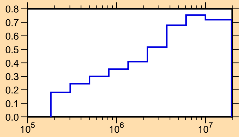
\mu vs. E for ^{42}\text{S}(\text{mt251})
