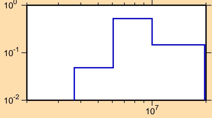
\sigma vs. E for ^{42}\text{S}(n,n\text{cont.})
