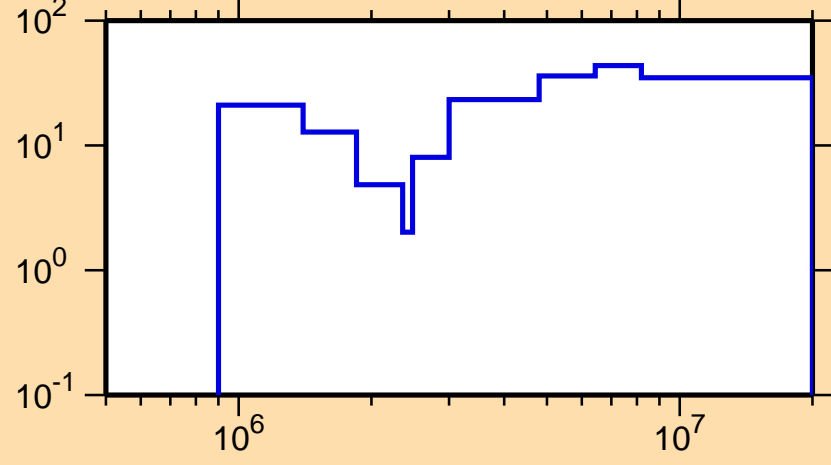
\Delta\sigma/\sigma vs. E for ^{42}\text{S}(n,\text{el.})
