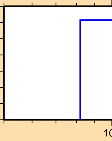
\sigma vs. E for ^{42}\text{S}(n,d)
