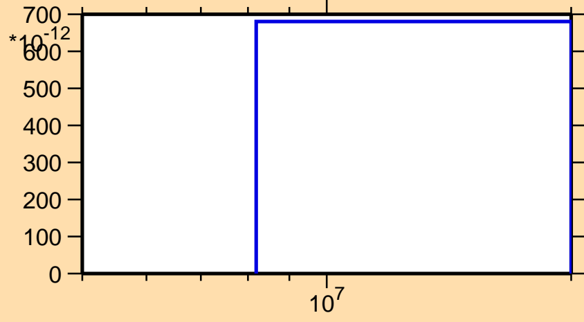
\sigma vs. E for ^{42}\text{S}(n,t)
