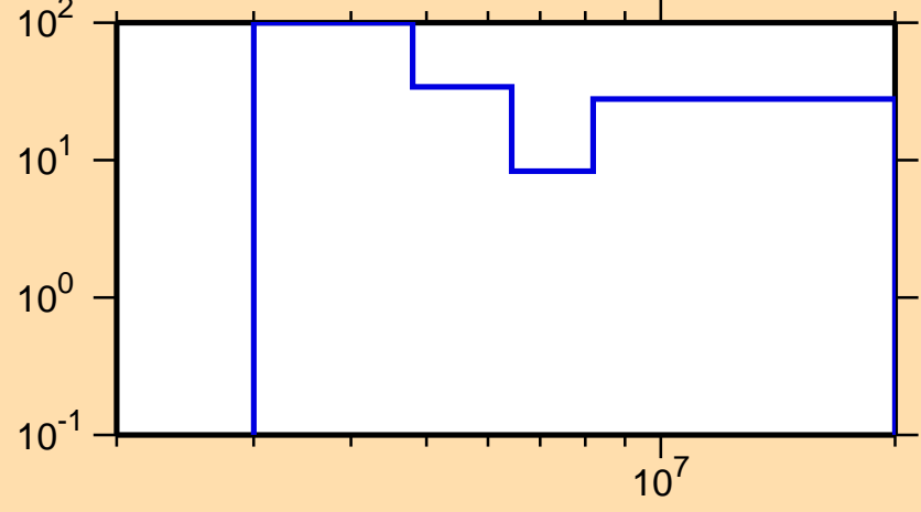
\Delta\sigma/\sigma vs. E for ^{42}\text{S}(n,ncont.)
