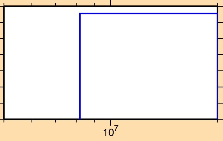
\sigma vs. E for ^{42}\text{S}(n,3n)
