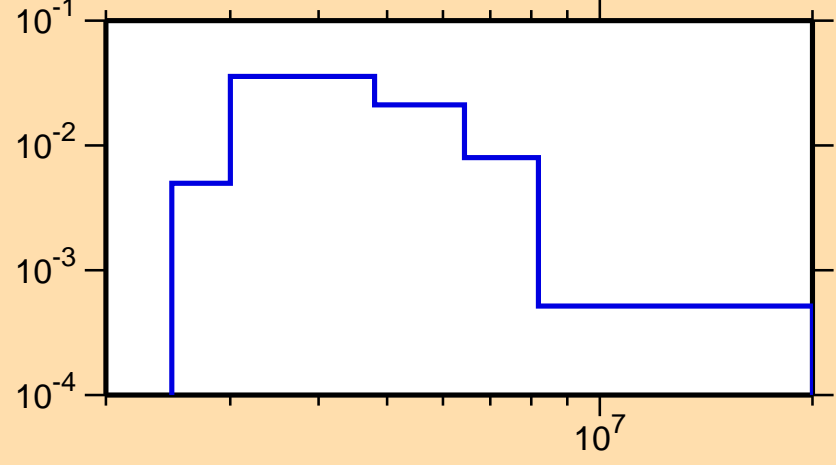
\sigma vs. E for ^{42}\text{S}(n,n_4)
