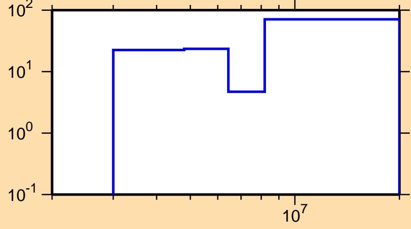
\Delta\sigma/\sigma vs. E for ^{42}\text{S}(n,\text{inel.})
