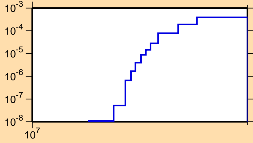
\sigma vs. E for ^{105}\text{Sb}(n,2np)
