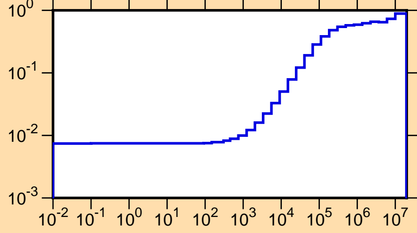
\mu vs. E for ^{105}\text{Sb}(\text{mt251})
