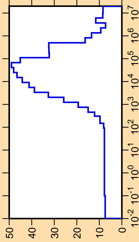
\Delta\mu/\mu vs. E for ^{105}\text{Sb}(\text{mt251})
