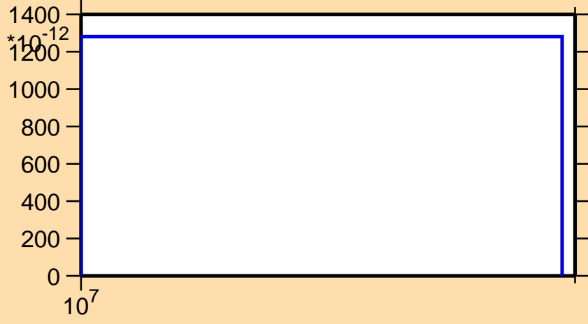
\sigma vs. E for ^{105}\text{Sb} (mt 34)
