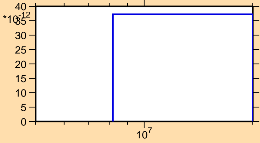
\sigma vs. E for ^{105}\text{Sb}(n,nt)
