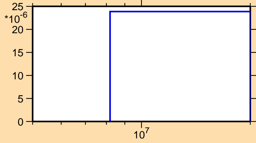
\sigma vs. E for ^{105}\text{Sb}(n,2np)
