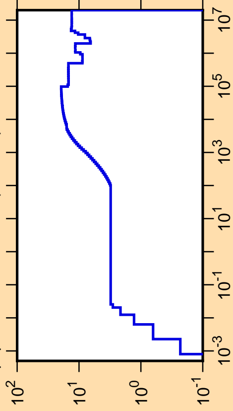
\Delta\mu/\mu vs. E for ^{107}\text{Sb}(\text{mt251})
