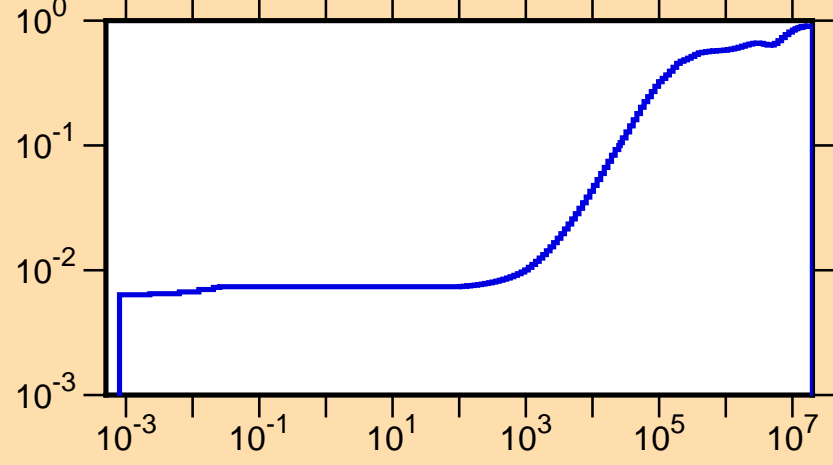
\mu vs. E for ^{107}\text{Sb}(\text{mt251})
