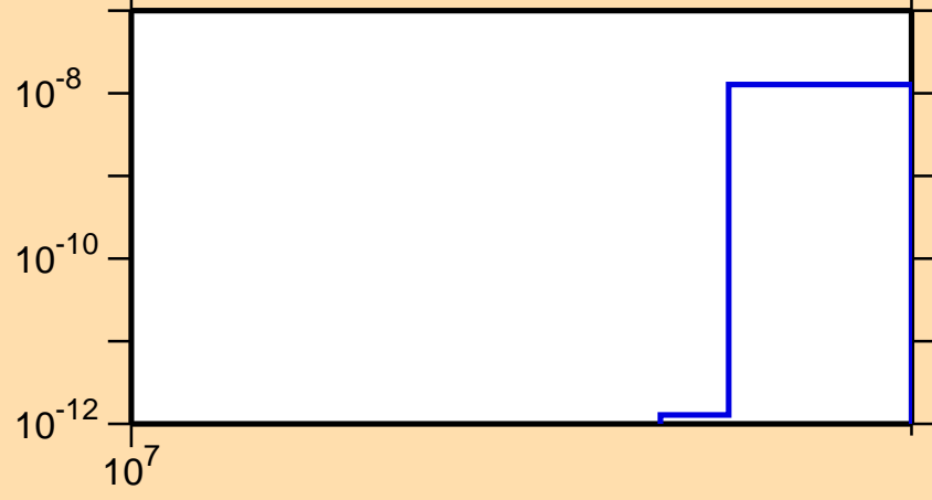
\sigma vs. E for ^{107}\text{Sb}(n,nt)
