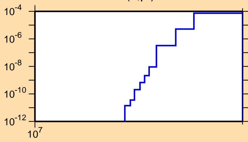
\sigma vs. E for ^{107}\text{Sb}(n,\text{pt})
