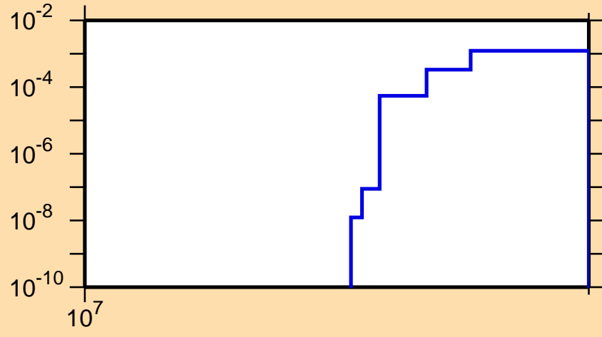
\sigma vs. E for ^{107}\text{Sb}(n,2np)
