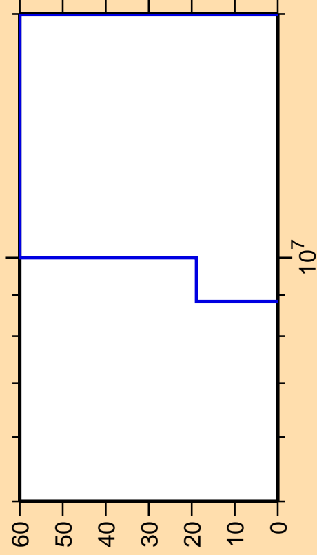
\Delta\sigma/\sigma vs. E for ^{108}\text{Sb} (mt 45)
