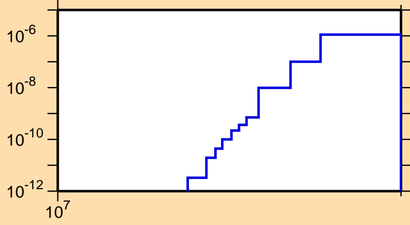
\sigma vs. E for ^{108}\text{Sb}(\text{mt } 34)
