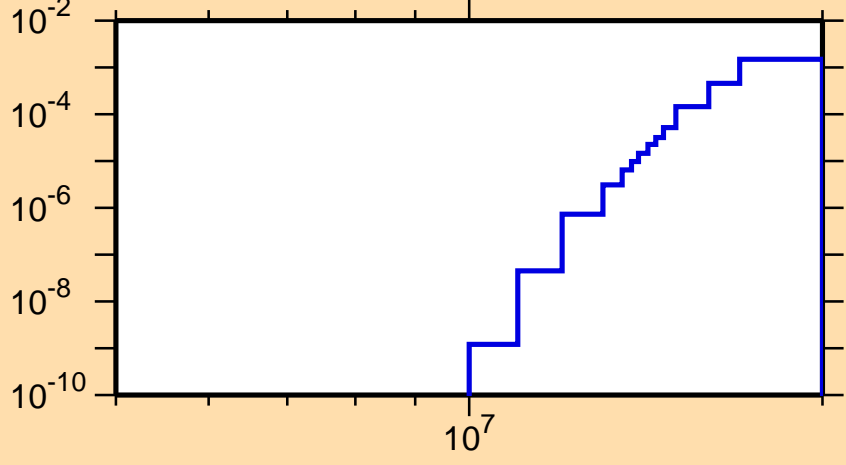
\sigma vs. E for ^{108}\text{Sb} (mt 45)
