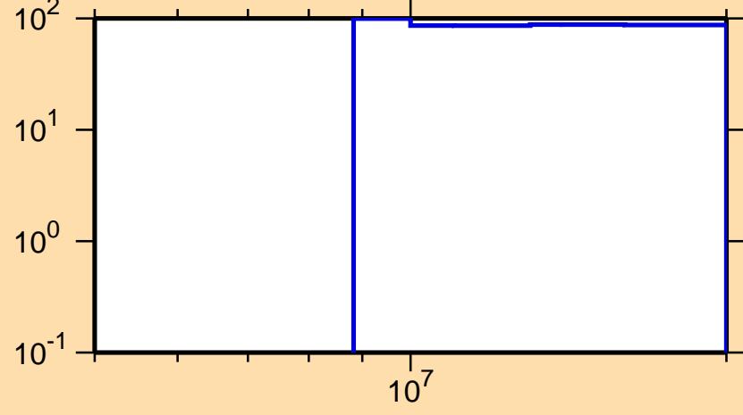
\Delta\sigma/\sigma vs. E for ^{108}\text{Sb}(n,2n)
