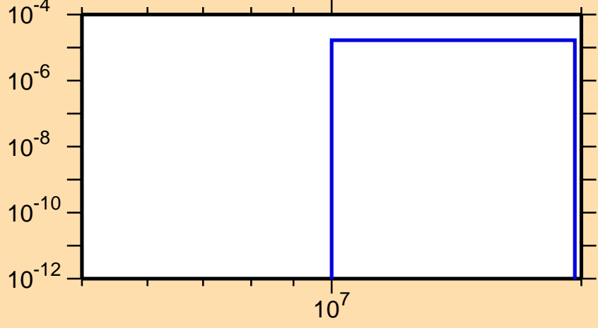
\sigma vs. E for ^{108}\text{Sb}(n,\text{pt})
