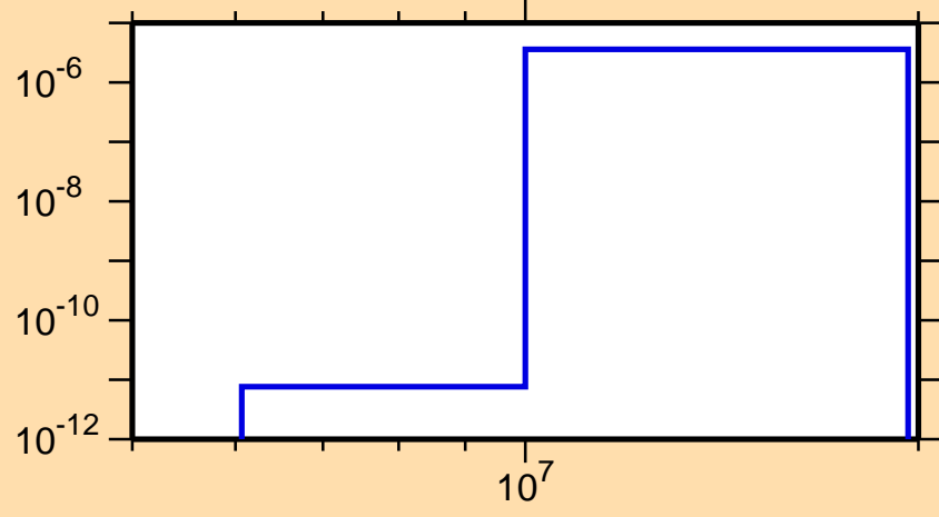
\sigma vs. E for ^{108}\text{Sb}(\text{mt117})
