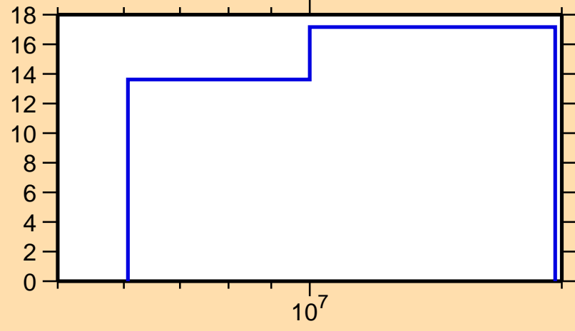
\Delta\sigma/\sigma vs. E for ^{108}\text{Sb}(n,\text{tot.})
