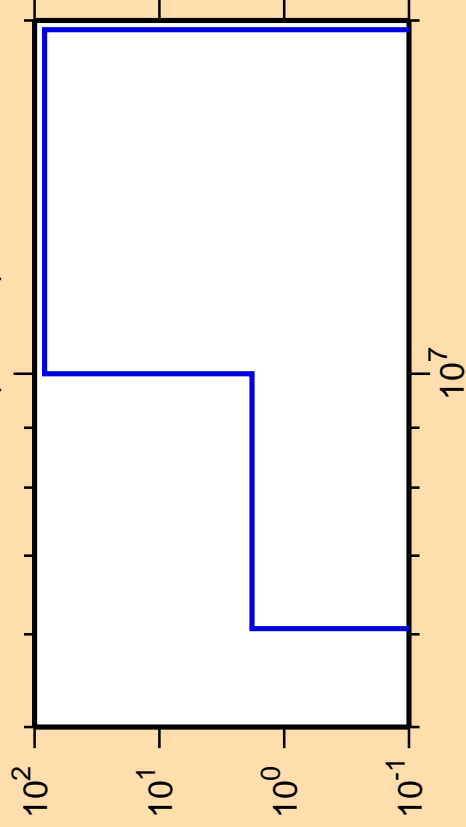
\Delta\sigma/\sigma vs. E for ^{108}\text{Sb}(\text{mt } 45)
