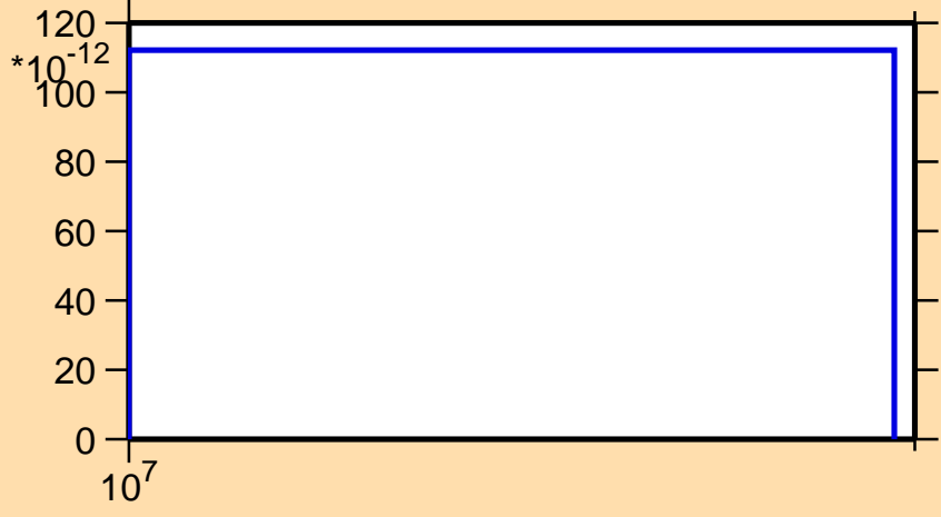
\sigma vs. E for ^{108}\text{Sb}(n,nt)
