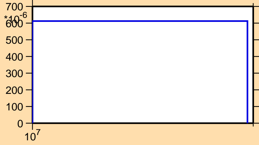
\sigma vs. E for ^{108}\text{Sb}(n,2np)
