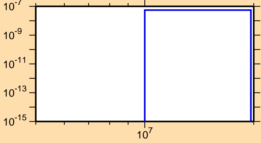
\sigma vs. E for ^{108}\text{Sb}(n,2n\alpha)
