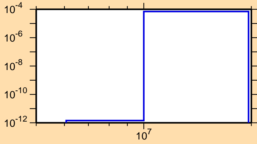
\sigma vs. E for ^{108}\text{Sb}(\text{mt } 45)
