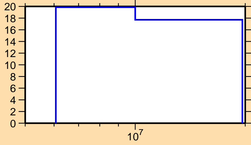
\Delta\sigma/\sigma vs. E for ^{108}\text{Sb}(n,\text{nonel.})
