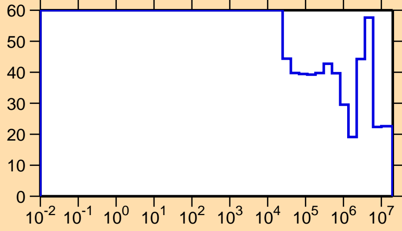
\Delta\sigma/\sigma vs. E for ^{108}\text{Sb}(n,\text{el.})
