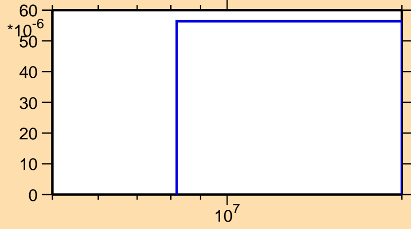
\sigma vs. E for ^{108}\text{Sb}(\text{mt } 45)
