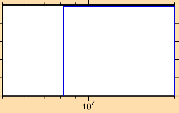
\sigma vs. E for ^{108}\text{Sb}(n,2np)
