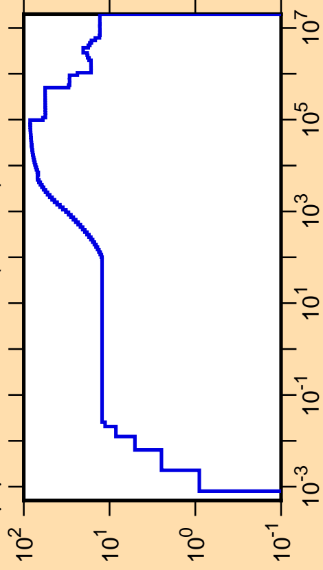
\Delta\mu/\mu vs. E for ^{111}\text{Sb}(\text{mt251})
