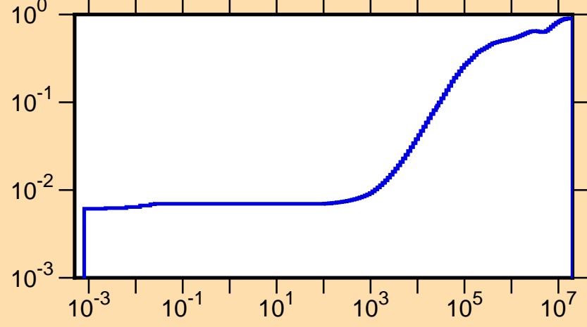
\mu vs. E for ^{111}\text{Sb}(\text{mt251})
