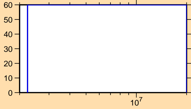
\Delta\sigma/\sigma vs. E for ^{111}\text{Sb}(n,n\text{cont.})
