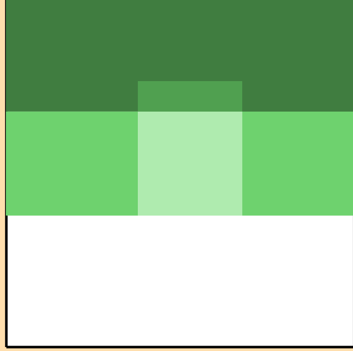
\Delta\sigma/\sigma vs. E for ^{111}\text{Sb}(n,\text{nonel.})
