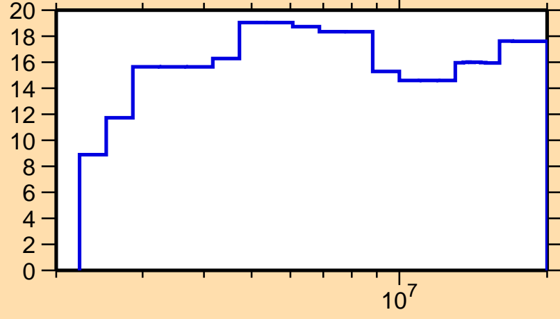
\Delta\sigma/\sigma vs. E for ^{111}\text{Sb}(n,n\text{nonel.})
