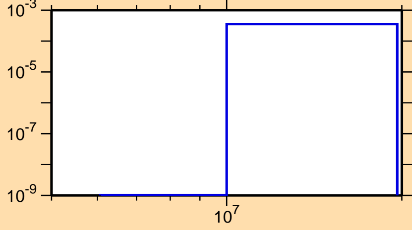
\sigma vs. E for ^{111}\text{Sb}(n,t)
