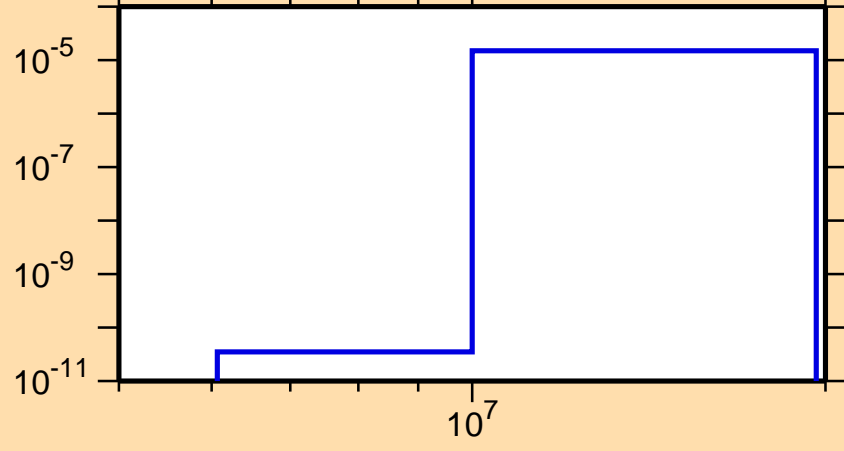
\sigma vs. E for ^{111}\text{Sb}(n,\text{He3})
