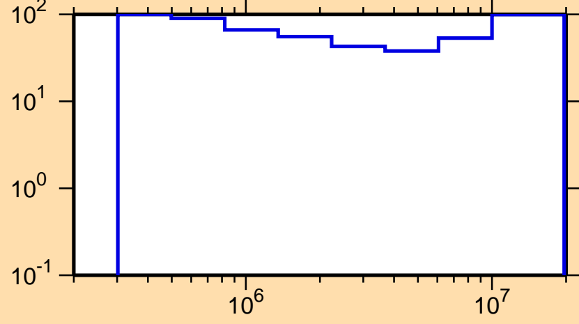
\Delta\sigma/\sigma vs. E for ^{111}\text{Sb}(n,n_1)
