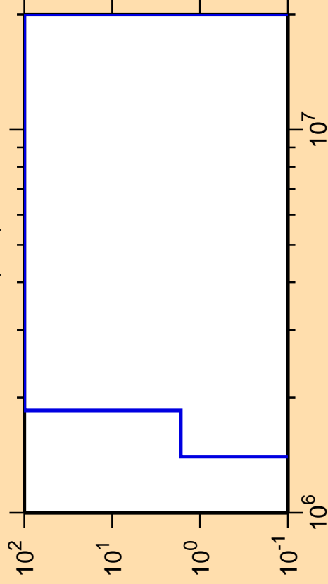
\Delta\sigma/\sigma vs. E for ^{111}\text{Sb}(n,d)
