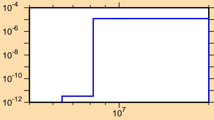
\sigma vs. E for ^{111}\text{Sb}(n,\text{He3})
