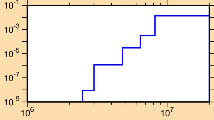
\sigma vs. E for ^{111}\text{Sb}(n,d)
