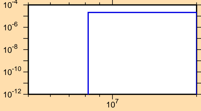
\sigma vs. E for ^{112}\text{Sb}(n,\text{He3})
