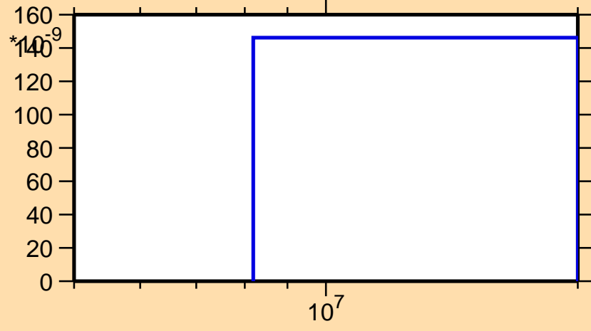
\sigma vs. E for ^{112}\text{Sb}(n,\text{pd})
