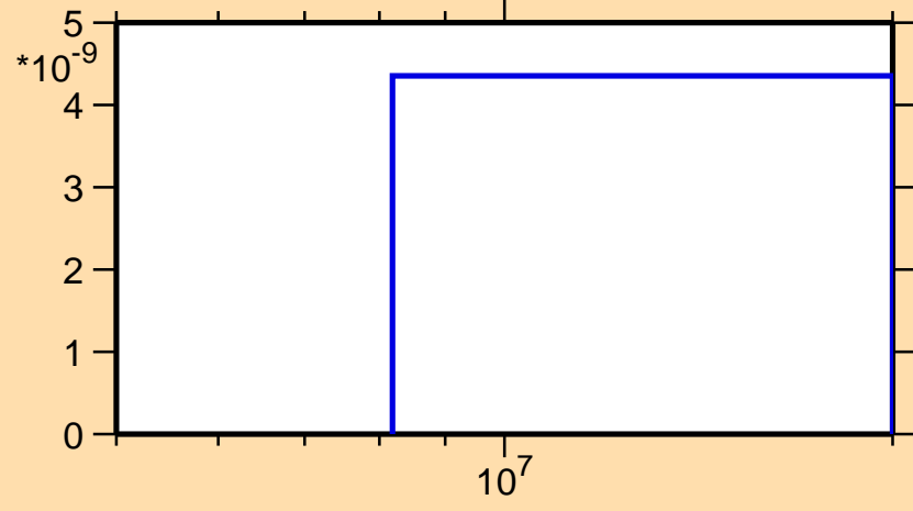
\sigma vs. E for ^{112}\text{Sb}(\text{mt117})
