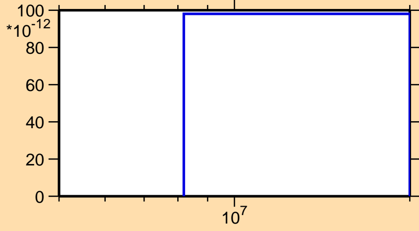
\sigma vs. E for ^{112}\text{Sb}(\text{mt } 34)
