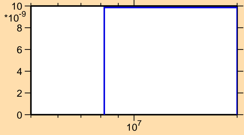
\sigma vs. E for ^{112}\text{Sb}(n,\text{pt})
