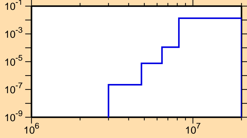
\sigma vs. E for ^{112}\text{Sb}(n,d)
