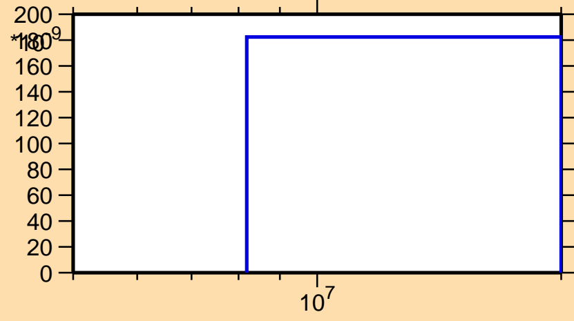
\sigma vs. E for ^{112}\text{Sb}(\text{mt } 45)
