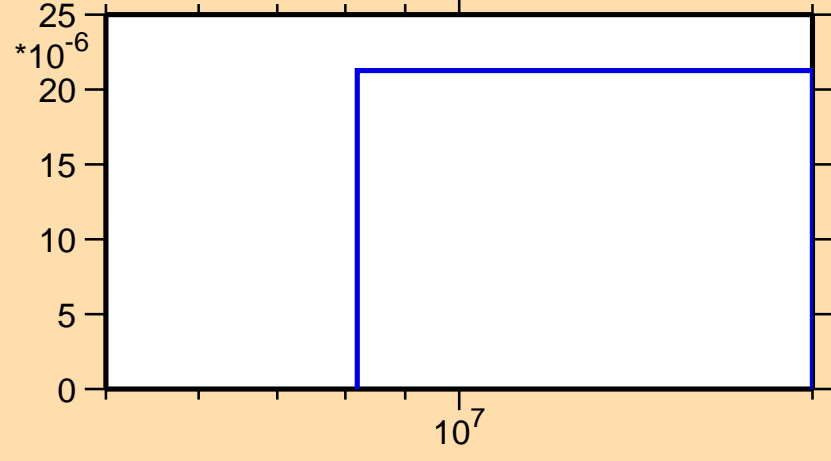
\sigma vs. E for ^{112}\text{Sb}(n,nd)
