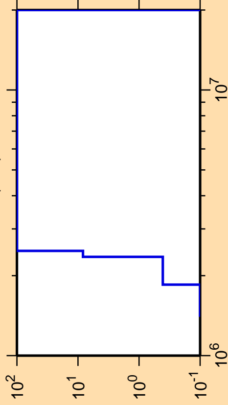
\Delta\sigma/\sigma vs. E for ^{112}\text{Sb}(n,d)
