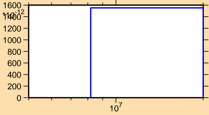
\sigma vs. E for ^{112}\text{Sb}(n,nt)
