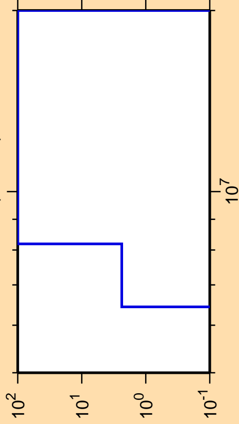
\Delta\sigma/\sigma vs. E for ^{112}\text{Sb}(n,\text{He3})
