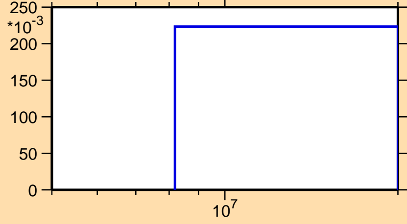
\sigma vs. E for ^{112}\text{Sb}(n,2n)
