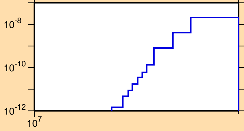
\sigma vs. E for ^{113}\text{Sb}(\text{mt117})
