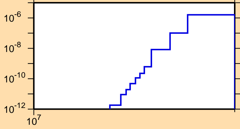
\sigma vs. E for ^{113}\text{Sb} (mt 45)
