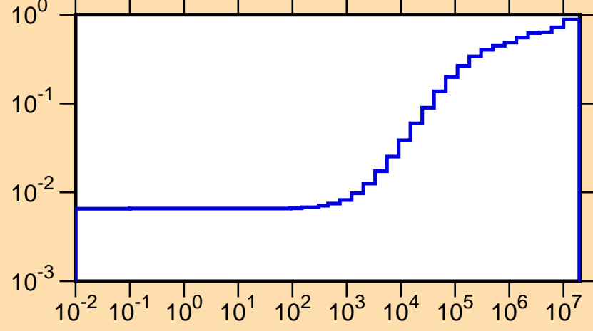
\mu vs. E for ^{113}\text{Sb}(\text{mt251})
