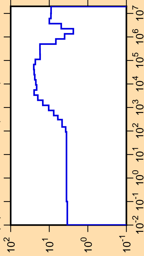
\Delta\mu/\mu vs. E for ^{113}\text{Sb}(\text{mt251})
