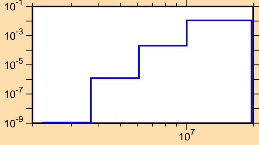
\sigma vs. E for ^{113}\text{Sb}(n,d)
