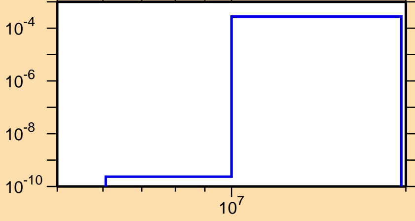
\sigma vs. E for ^{113}\text{Sb}(n,t)
