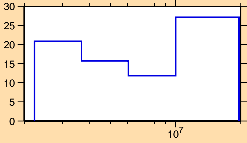
\Delta\sigma/\sigma vs. E for ^{113}\text{Sb}(n,ncont.)
