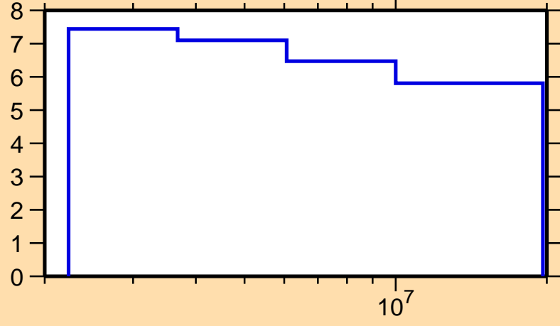
\Delta\sigma/\sigma vs. E for ^{113}\text{Sb}(n,\text{nonel.})
