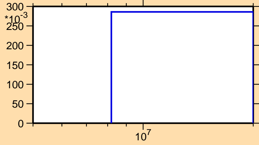
\sigma vs. E for ^{113}\text{Sb}(n,2n)
