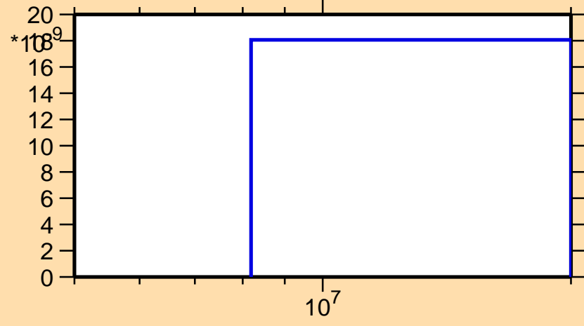
\sigma vs. E for ^{113}\text{Sb}(\text{mt } 45)
