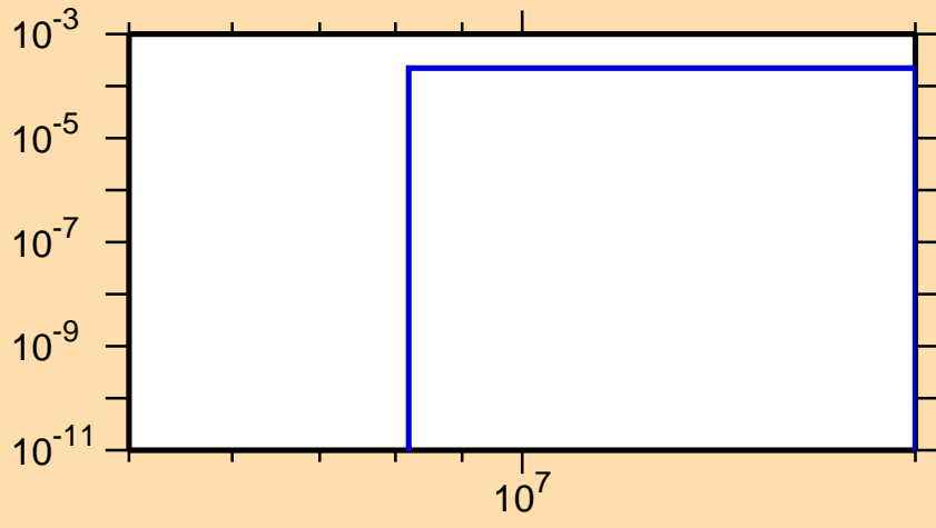
\sigma vs. E for ^{113}\text{Sb}(n,t)
