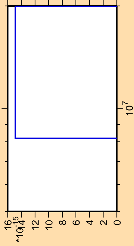
\Delta\sigma/\sigma vs. E for ^{113}\text{Sb} (mt 11)
