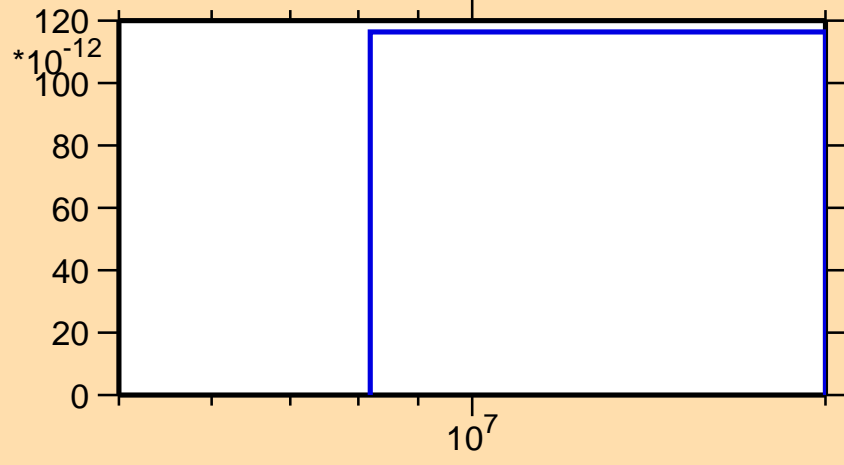
\sigma vs. E for ^{113}\text{Sb}(n,3n)
