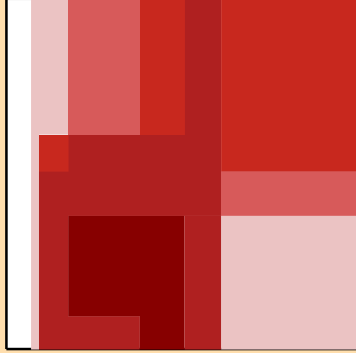
\Delta\sigma/\sigma vs. E for ^{113}\text{Sb}(n,ncont.)
