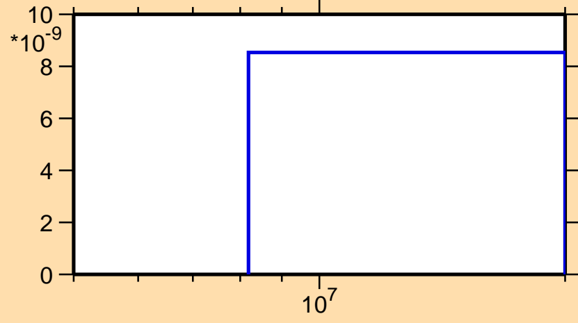
\sigma vs. E for ^{113}\text{Sb}(n,\text{pd})
