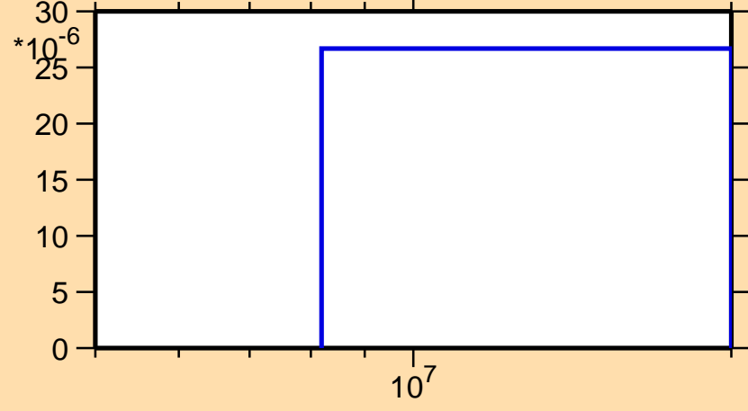
\sigma vs. E for ^{113}\text{Sb}(n,2np)
