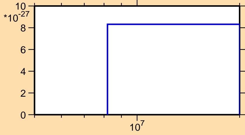
\sigma vs. E for ^{113}\text{Sb} (mt 11)
