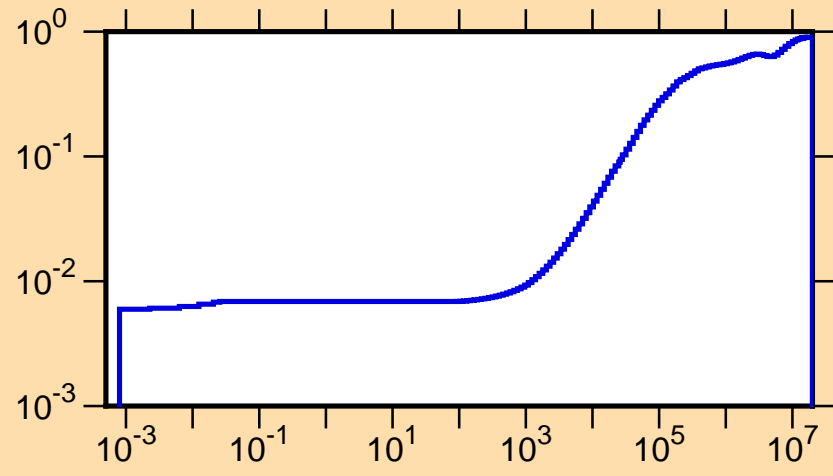
\mu vs. E for ^{114}\text{Sb}(\text{mt251})
