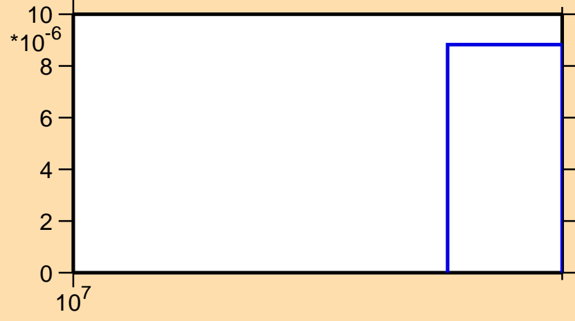
\sigma vs. E for ^{114}\text{Sb}(n,3n)
