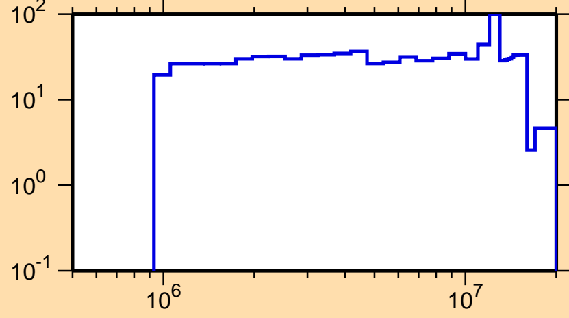
\Delta\sigma/\sigma vs. E for ^{114}\text{Sb}(n,n_1)
